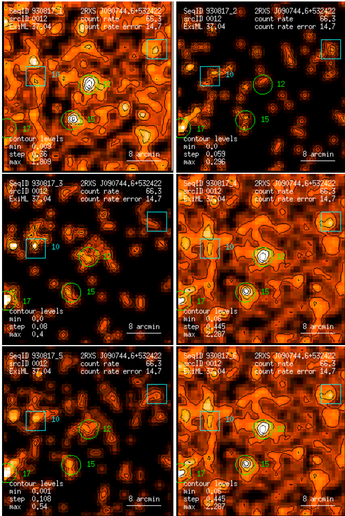
Figure 12: RASS 930817: detection 0012: band rate images, Gaussian filter: (1) PSPC channels 11 – 41, (2) 52 – 90, (3) 91 – 201, (4) 11 – 235, (5) 52 – 201, (6) 11 – 201. Broad band rates in counts/ks. Band rate contour levels in counts/ks/arcmin 2 .
