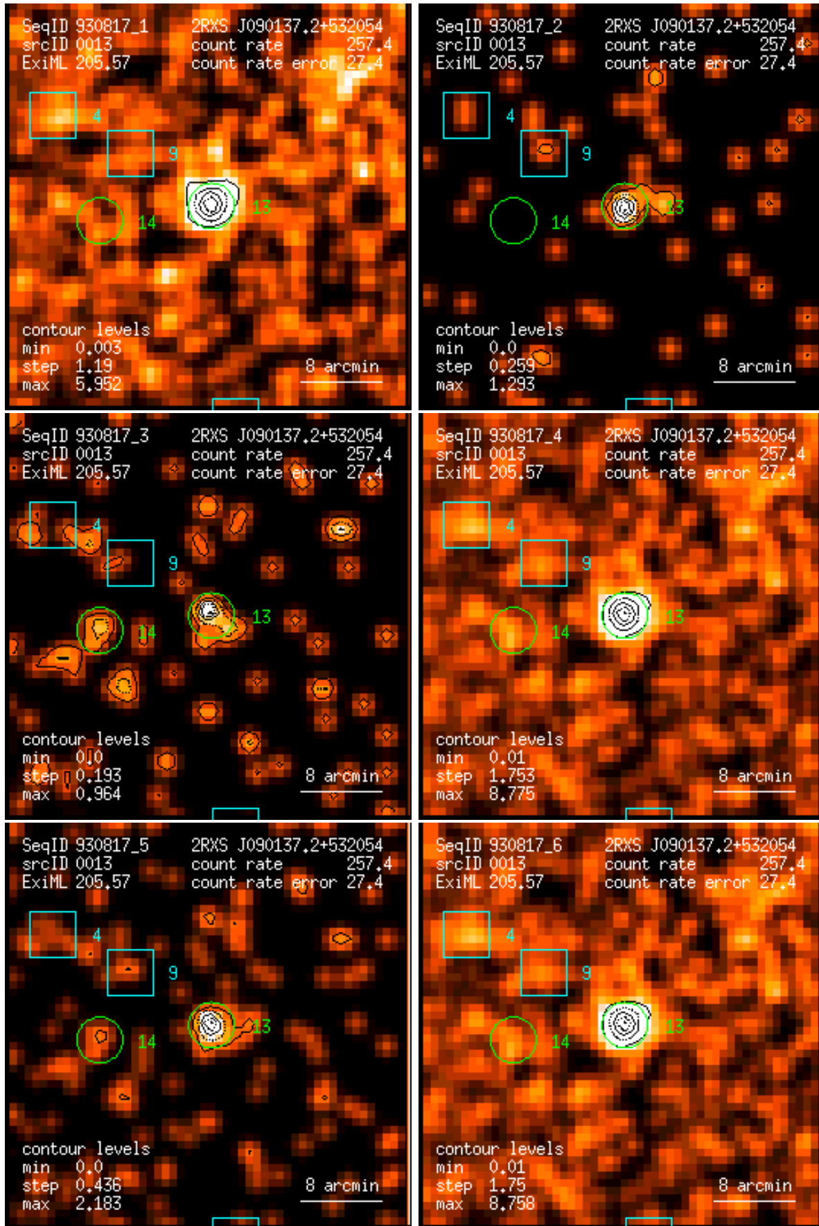
Figure 13: RASS 930817: detection 0013: band rate images, Gaussian filter: (1) PSPC channels 11 – 41, (2) 52 – 90, (3) 91 – 201, (4) 11 – 235, (5) 52 – 201, (6) 11 – 201. Broad band rates in counts/ks. Band rate contour levels in counts/ks/arcmin 2 .
