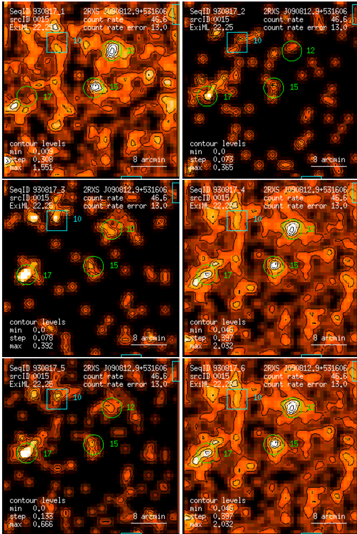
Figure 15: RASS 930817: detection 0015: band rate images, Gaussian filter: (1) PSPC channels 11 – 41, (2) 52 – 90, (3) 91 – 201, (4) 11 – 235, (5) 52 – 201, (6) 11 – 201. Broad band rates in counts/ks. Band rate contour levels in counts/ks/arcmin 2 .
