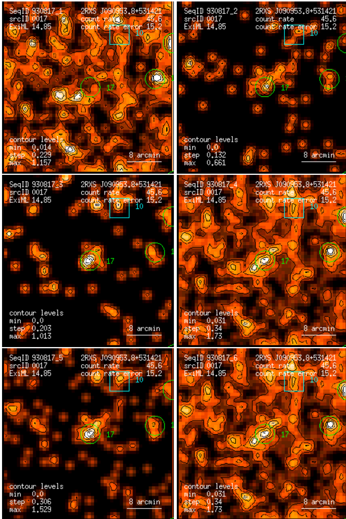
Figure 17: RASS 930817: detection 0017: band rate images, Gaussian filter: (1) PSPC channels 11 – 41, (2) 52 – 90, (3) 91 – 201, (4) 11 – 235, (5) 52 – 201, (6) 11 – 201. Broad band rates in counts/ks. Band rate contour levels in counts/ks/arcmin 2 .
