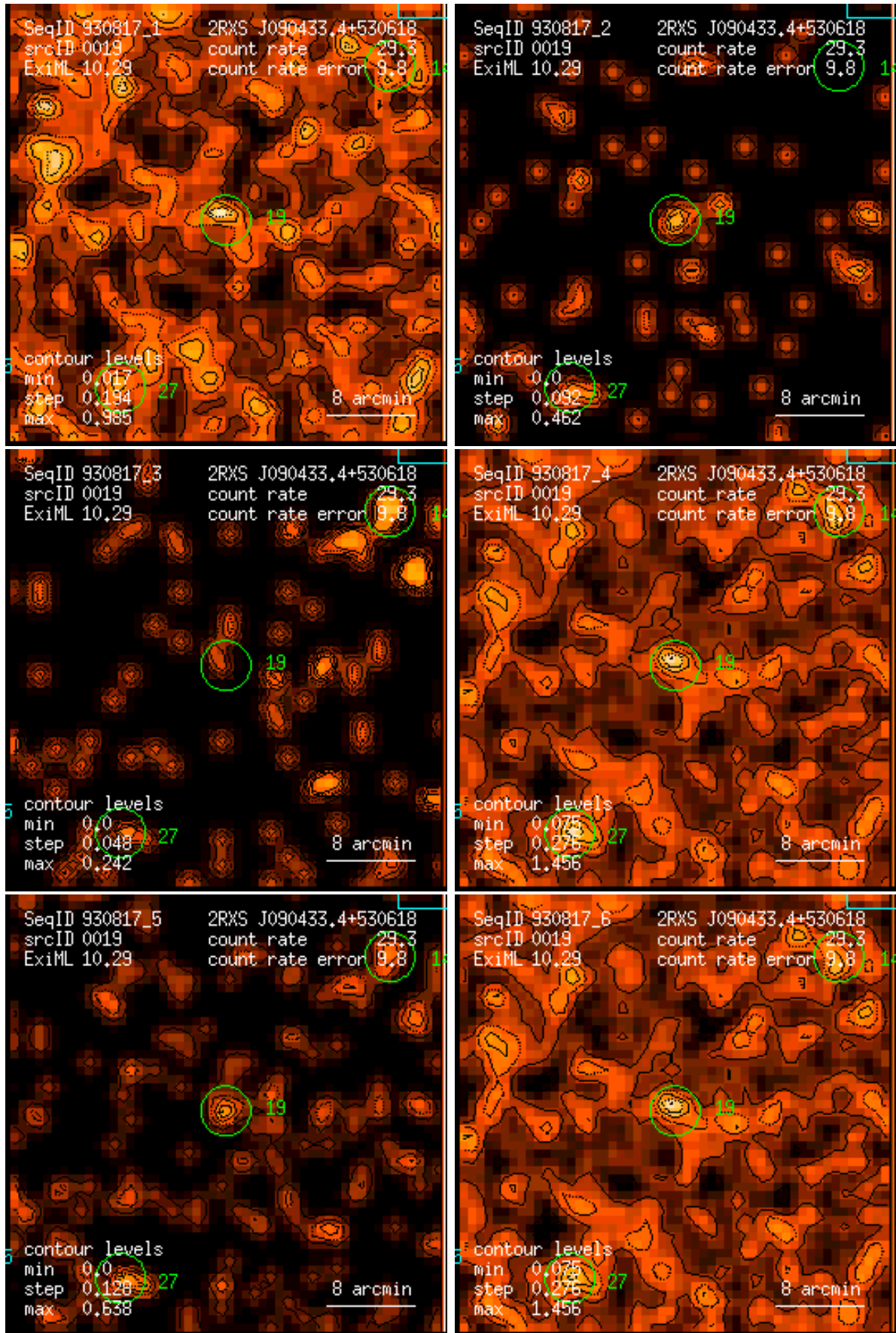
Figure 19: RASS 930817: detection 0019: band rate images, Gaussian filter: (1) PSPC channels 11 – 41, (2) 52 – 90, (3) 91 – 201, (4) 11 – 235, (5) 52 – 201, (6) 11 – 201. Broad band rates in counts/ks. Band rate contour levels in counts/ks/arcmin 2 .
