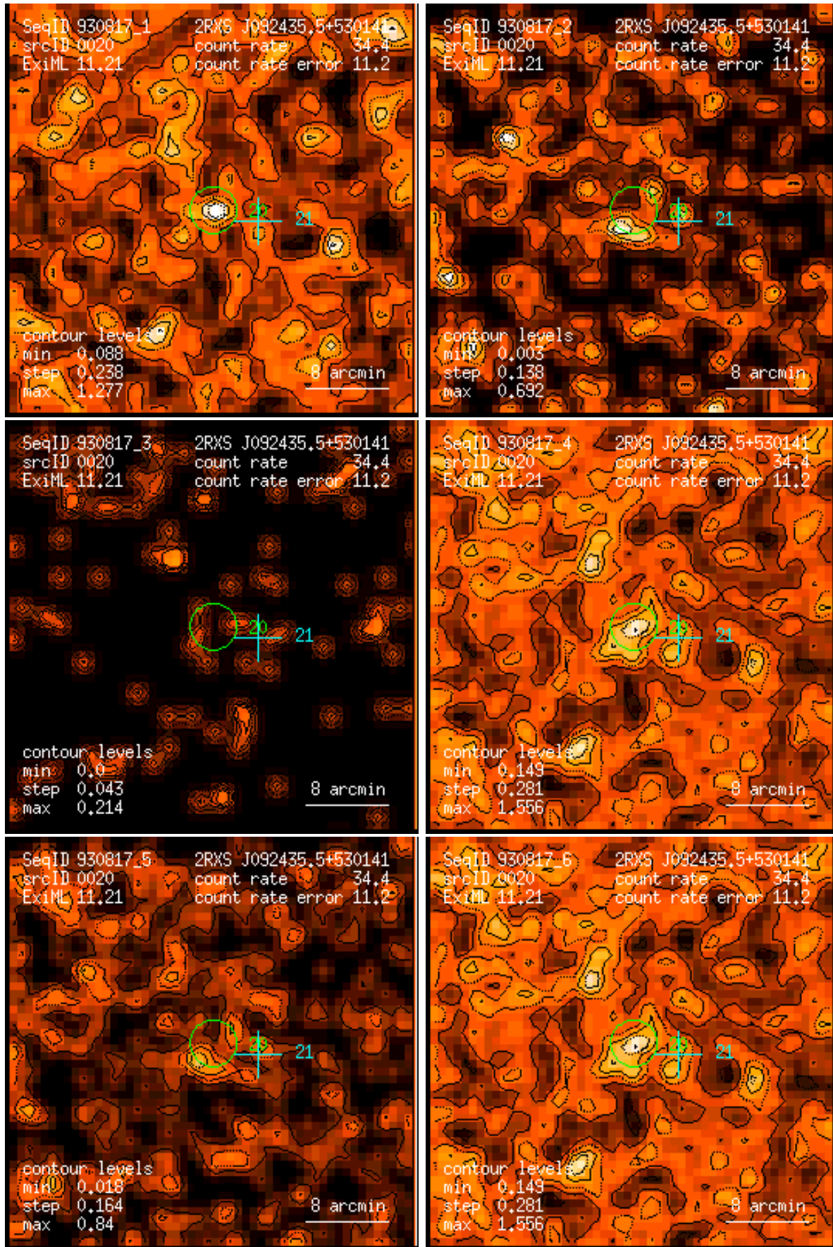
Figure 20: RASS 930817: detection 0020: band rate images, Gaussian filter: (1) PSPC channels 11 – 41, (2) 52 – 90, (3) 91 – 201, (4) 11 – 235, (5) 52 – 201, (6) 11 – 201. Broad band rates in counts/ks. Band rate contour levels in counts/ks/arcmin 2 .
