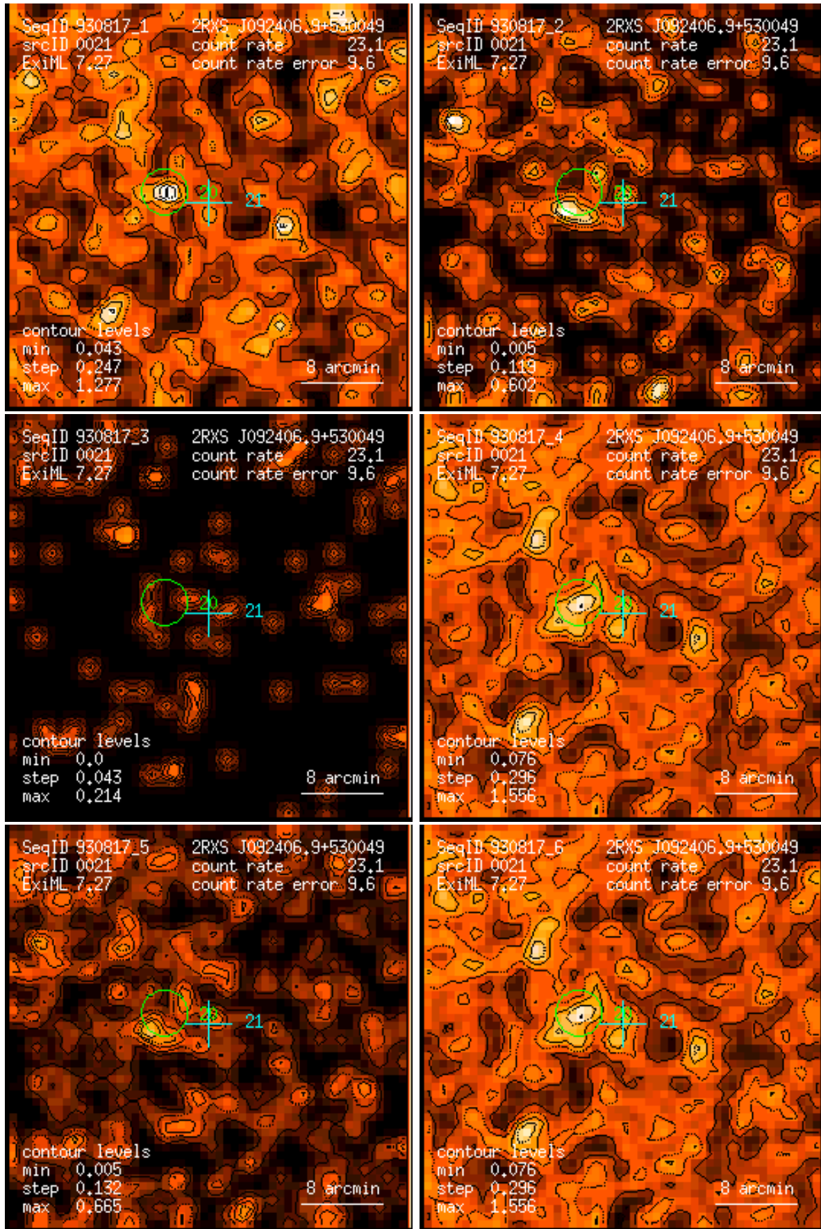
Figure 21: RASS 930817: detection 0021: band rate images, Gaussian filter: (1) PSPC channels 11 – 41, (2) 52 – 90, (3) 91 – 201, (4) 11 – 235, (5) 52 – 201, (6) 11 – 201. Broad band rates in counts/ks. Band rate contour levels in counts/ks/arcmin 2 .
