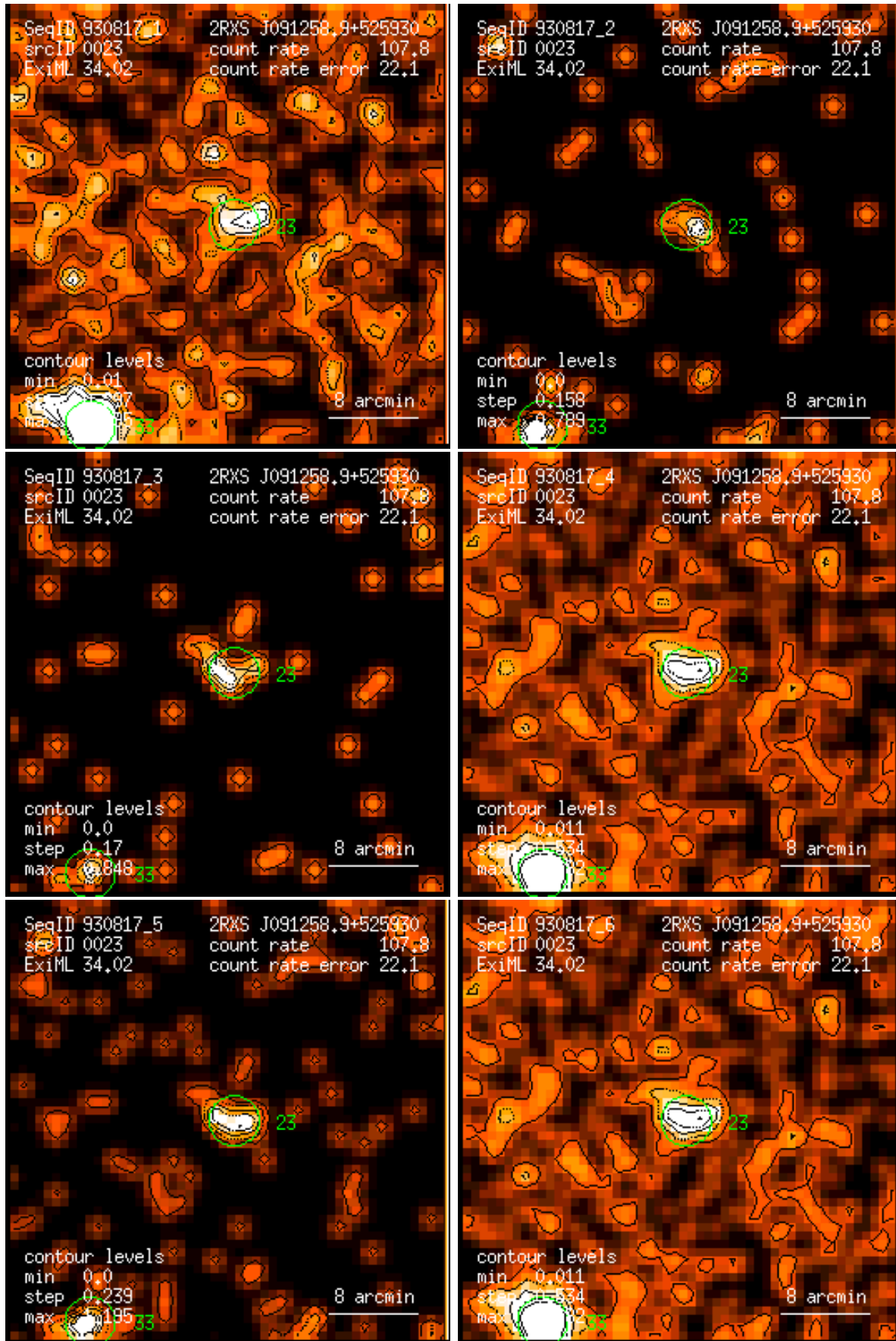
Figure 23: RASS 930817: detection 0023: band rate images, Gaussian filter: (1) PSPC channels 11 – 41, (2) 52 – 90, (3) 91 – 201, (4) 11 – 235, (5) 52 – 201, (6) 11 – 201. Broad band rates in counts/ks. Band rate contour levels in counts/ks/arcmin 2 .
