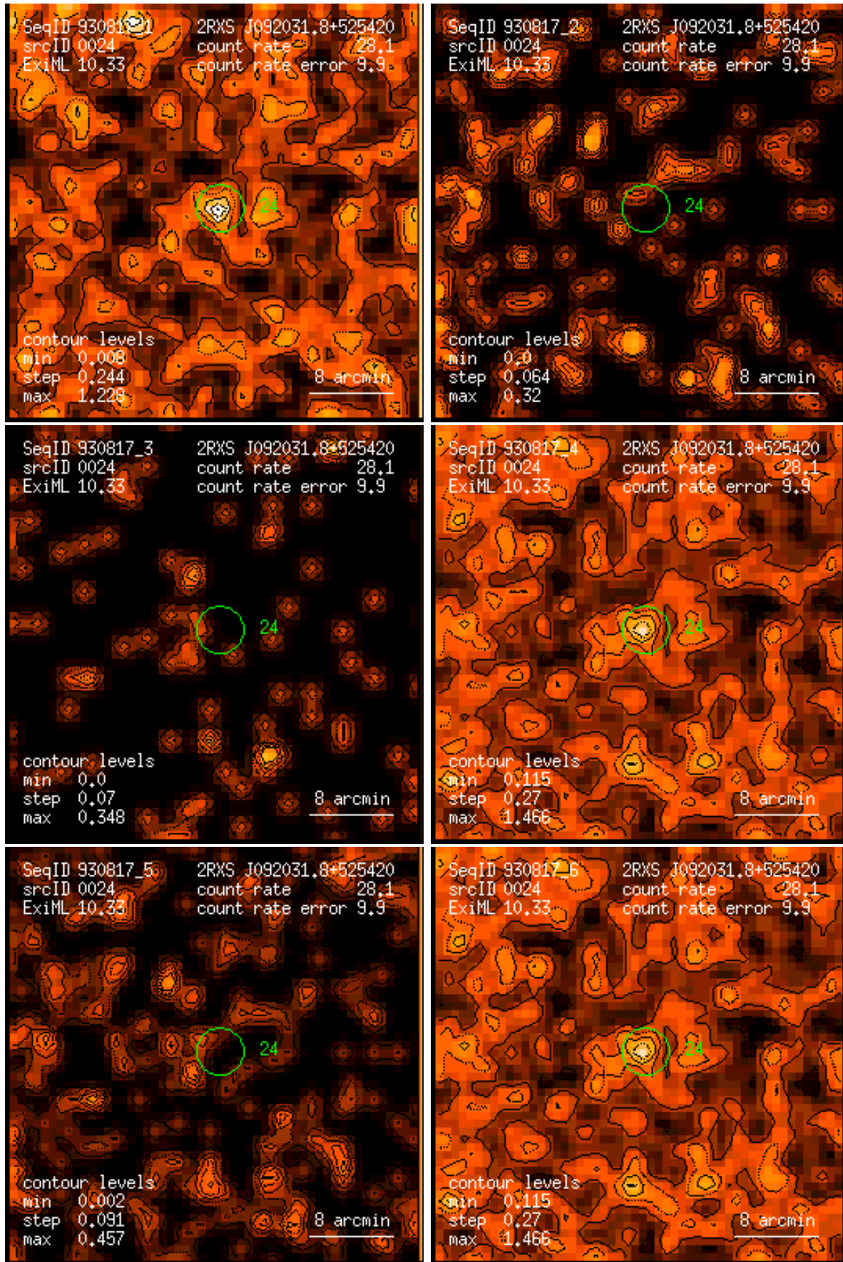
Figure 24: RASS 930817: detection 0024: band rate images, Gaussian filter: (1) PSPC channels 11 – 41, (2) 52 – 90, (3) 91 – 201, (4) 11 – 235, (5) 52 – 201, (6) 11 – 201. Broad band rates in counts/ks. Band rate contour levels in counts/ks/arcmin 2 .
