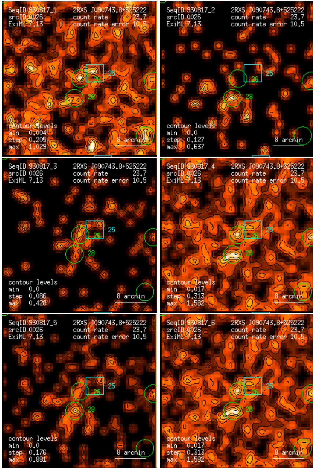
Figure 26: RASS 930817: detection 0026: band rate images, Gaussian filter: (1) PSPC channels 11 – 41, (2) 52 – 90, (3) 91 – 201, (4) 11 – 235, (5) 52 – 201, (6) 11 – 201. Broad band rates in counts/ks. Band rate contour levels in counts/ks/arcmin 2 .
