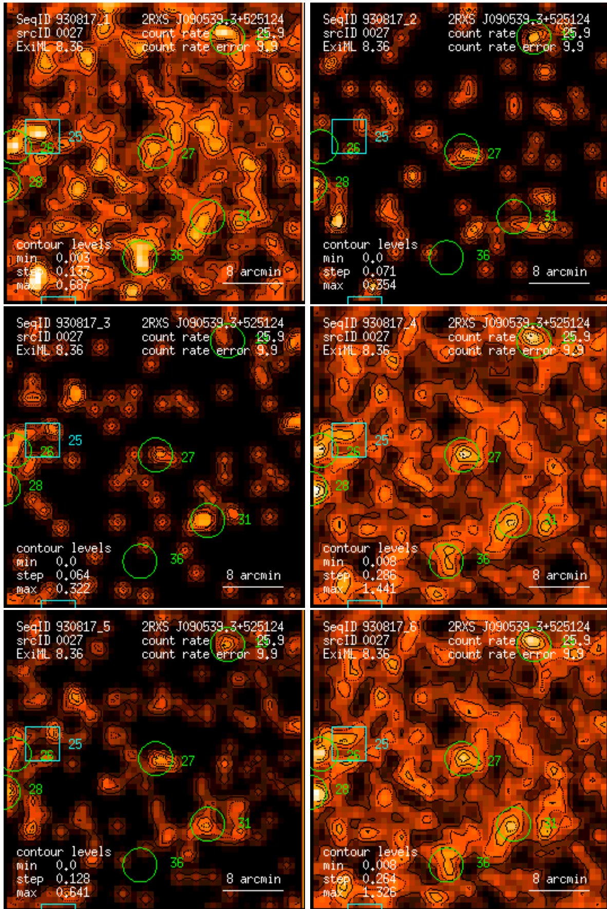
Figure 27: RASS 930817: detection 0027: band rate images, Gaussian filter: (1) PSPC channels 11 – 41, (2) 52 – 90, (3) 91 – 201, (4) 11 – 235, (5) 52 – 201, (6) 11 – 201. Broad band rates in counts/ks. Band rate contour levels in counts/ks/arcmin 2 .
