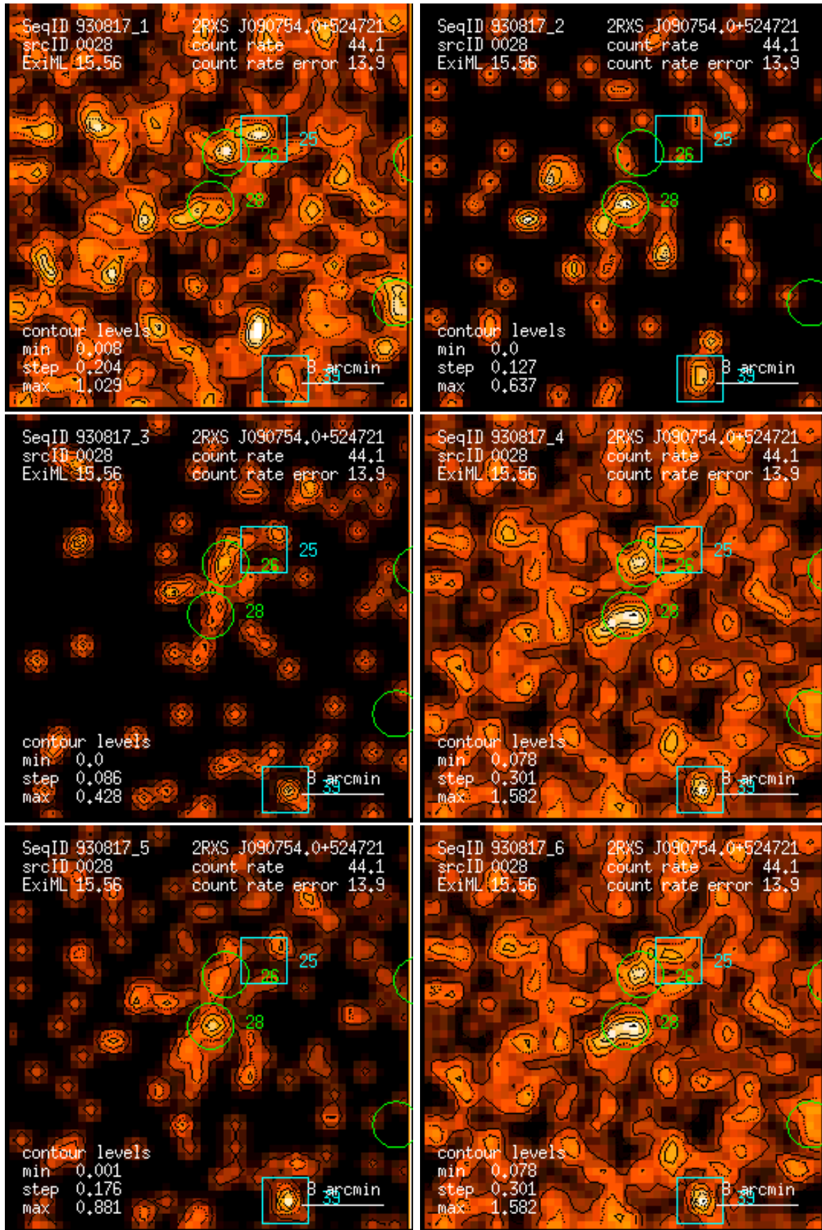
Figure 28: RASS 930817: detection 0028: band rate images, Gaussian filter: (1) PSPC channels 11 – 41, (2) 52 – 90, (3) 91 – 201, (4) 11 – 235, (5) 52 – 201, (6) 11 – 201. Broad band rates in counts/ks. Band rate contour levels in counts/ks/arcmin 2 .
