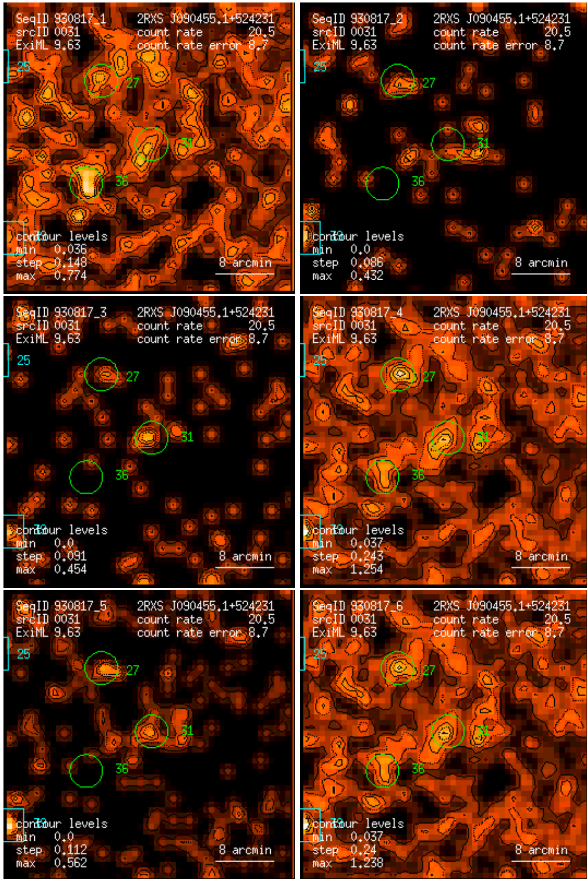
Figure 31: RASS 930817: detection 0031: band rate images, Gaussian filter: (1) PSPC channels 11 – 41, (2) 52 – 90, (3) 91 – 201, (4) 11 – 235, (5) 52 – 201, (6) 11 – 201. Broad band rates in counts/ks. Band rate contour levels in counts/ks/arcmin 2 .
