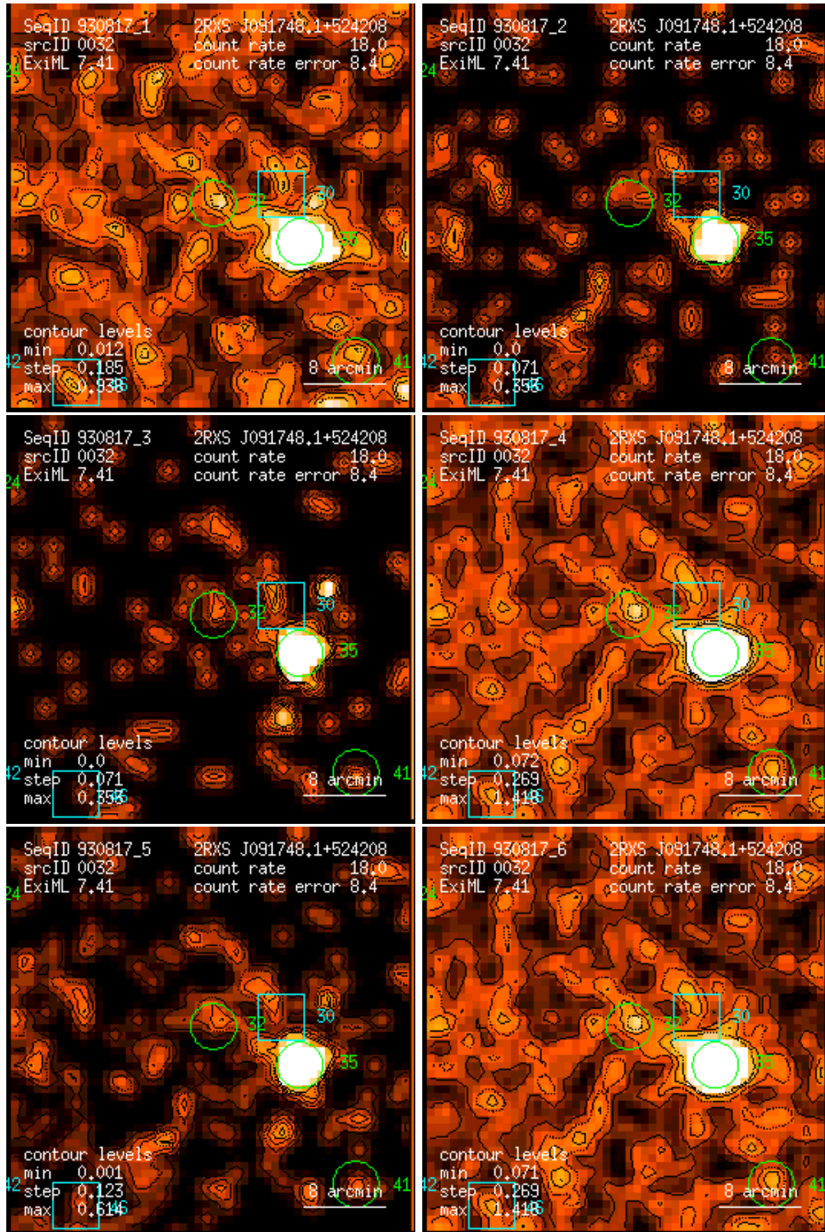
Figure 32: RASS 930817: detection 0032: band rate images, Gaussian filter: (1) PSPC channels 11 – 41, (2) 52 – 90, (3) 91 – 201, (4) 11 – 235, (5) 52 – 201, (6) 11 – 201. Broad band rates in counts/ks. Band rate contour levels in counts/ks/arcmin 2 .
