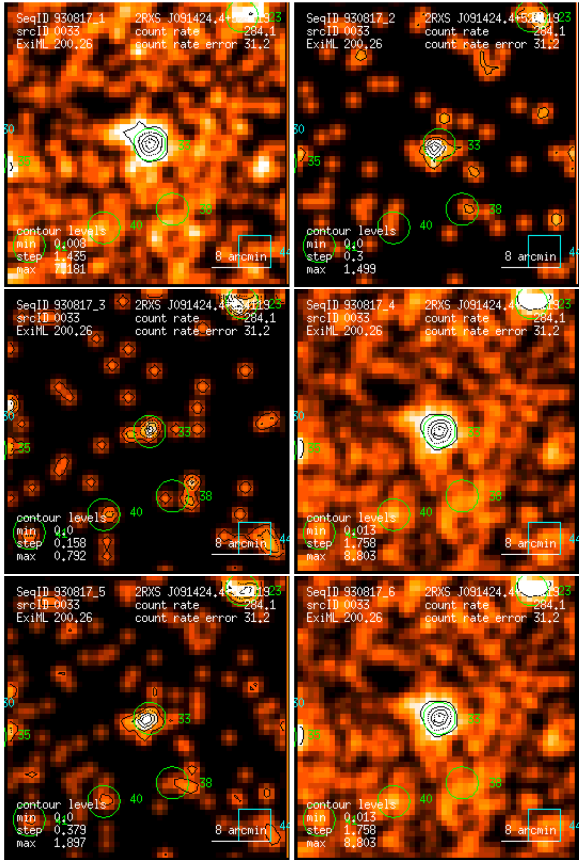
Figure 33: RASS 930817: detection 0033: band rate images, Gaussian filter: (1) PSPC channels 11 – 41, (2) 52 – 90, (3) 91 – 201, (4) 11 – 235, (5) 52 – 201, (6) 11 – 201. Broad band rates in counts/ks. Band rate contour levels in counts/ks/arcmin 2 .
