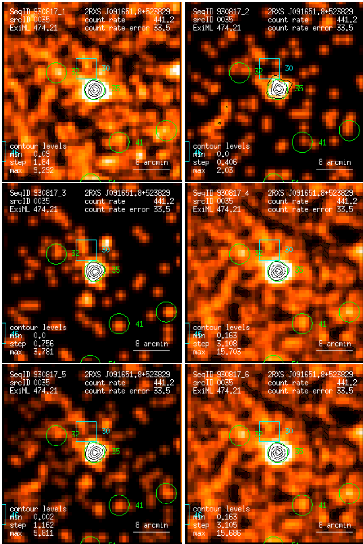
Figure 35: RASS 930817: detection 0035: band rate images, Gaussian filter: (1) PSPC channels 11 – 41, (2) 52 – 90, (3) 91 – 201, (4) 11 – 235, (5) 52 – 201, (6) 11 – 201. Broad band rates in counts/ks. Band rate contour levels in counts/ks/arcmin 2 .
