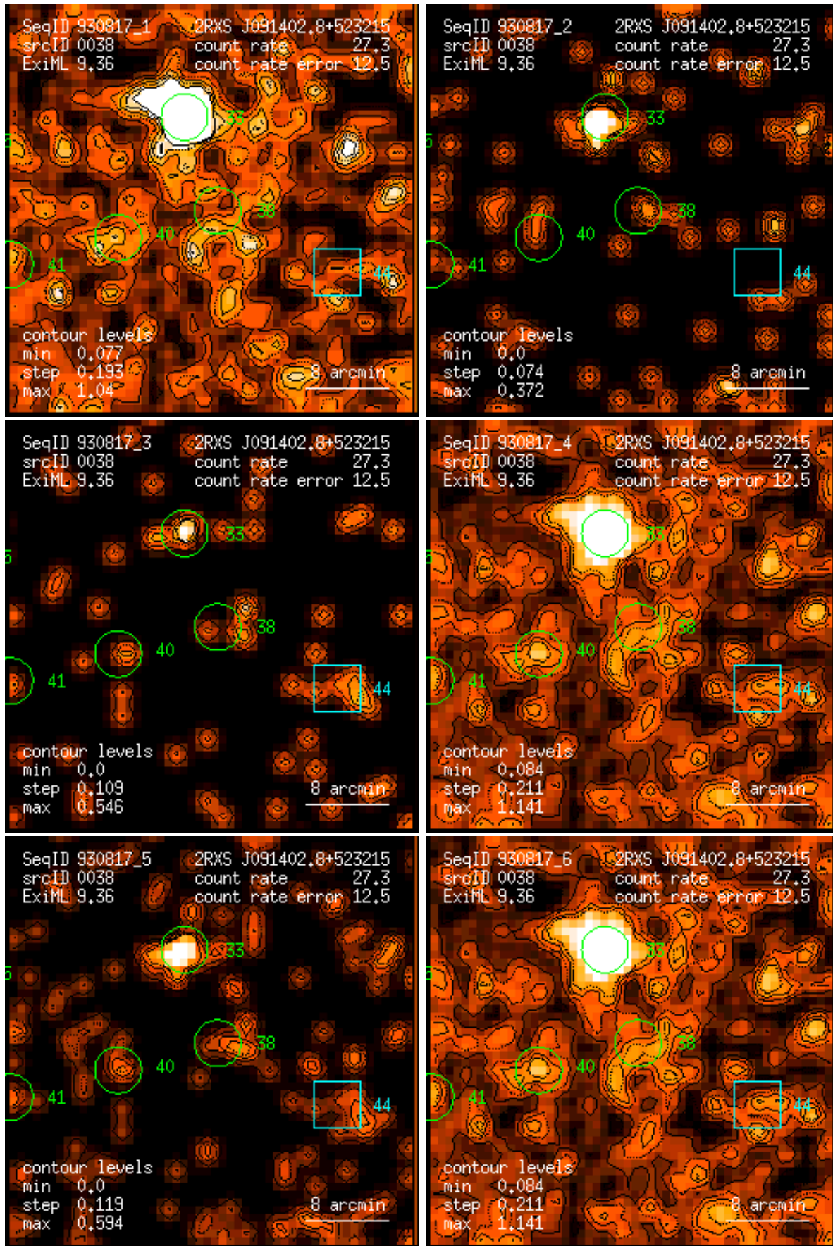
Figure 38: RASS 930817: detection 0038: band rate images, Gaussian filter: (1) PSPC channels 11 – 41, (2) 52 – 90, (3) 91 – 201, (4) 11 – 235, (5) 52 – 201, (6) 11 – 201. Broad band rates in counts/ks. Band rate contour levels in counts/ks/arcmin 2 .
