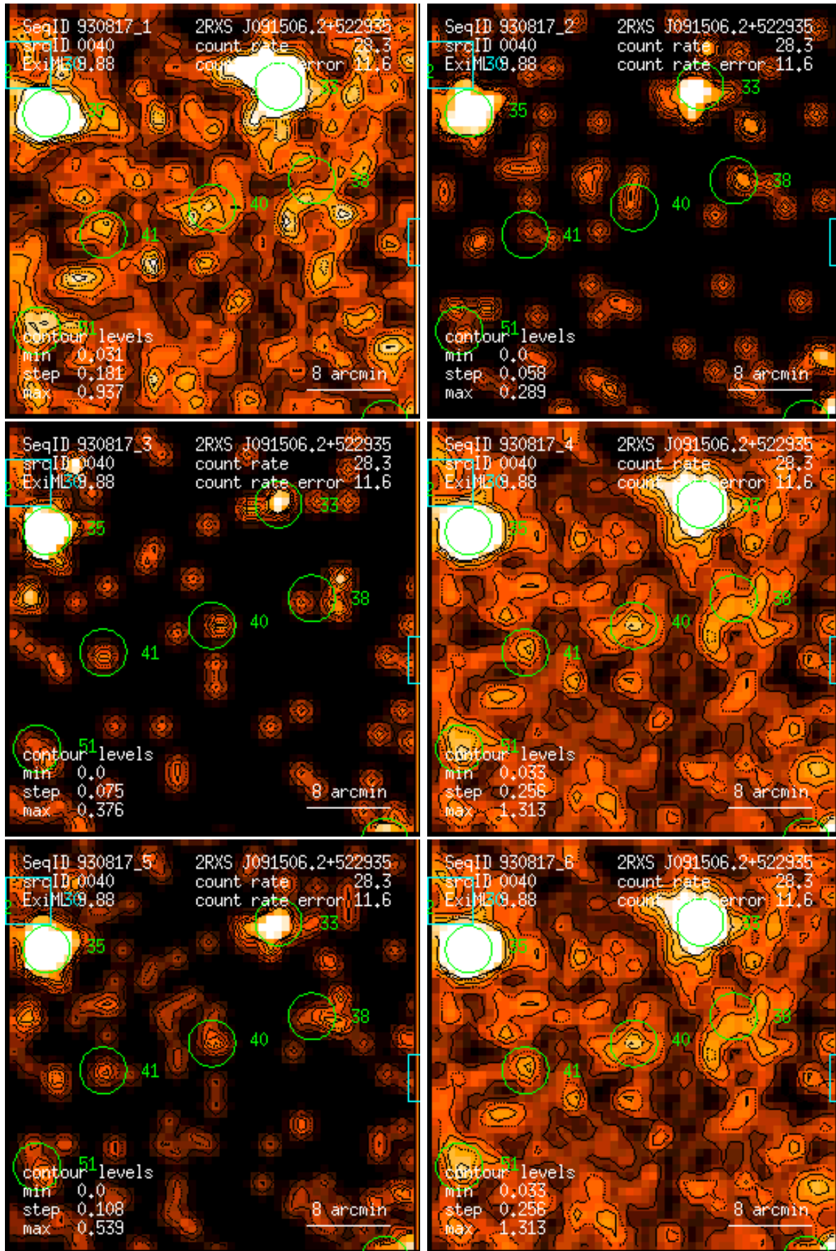
Figure 40: RASS 930817: detection 0040: band rate images, Gaussian filter: (1) PSPC channels 11 – 41, (2) 52 – 90, (3) 91 – 201, (4) 11 – 235, (5) 52 – 201, (6) 11 – 201. Broad band rates in counts/ks. Band rate contour levels in counts/ks/arcmin 2 .
