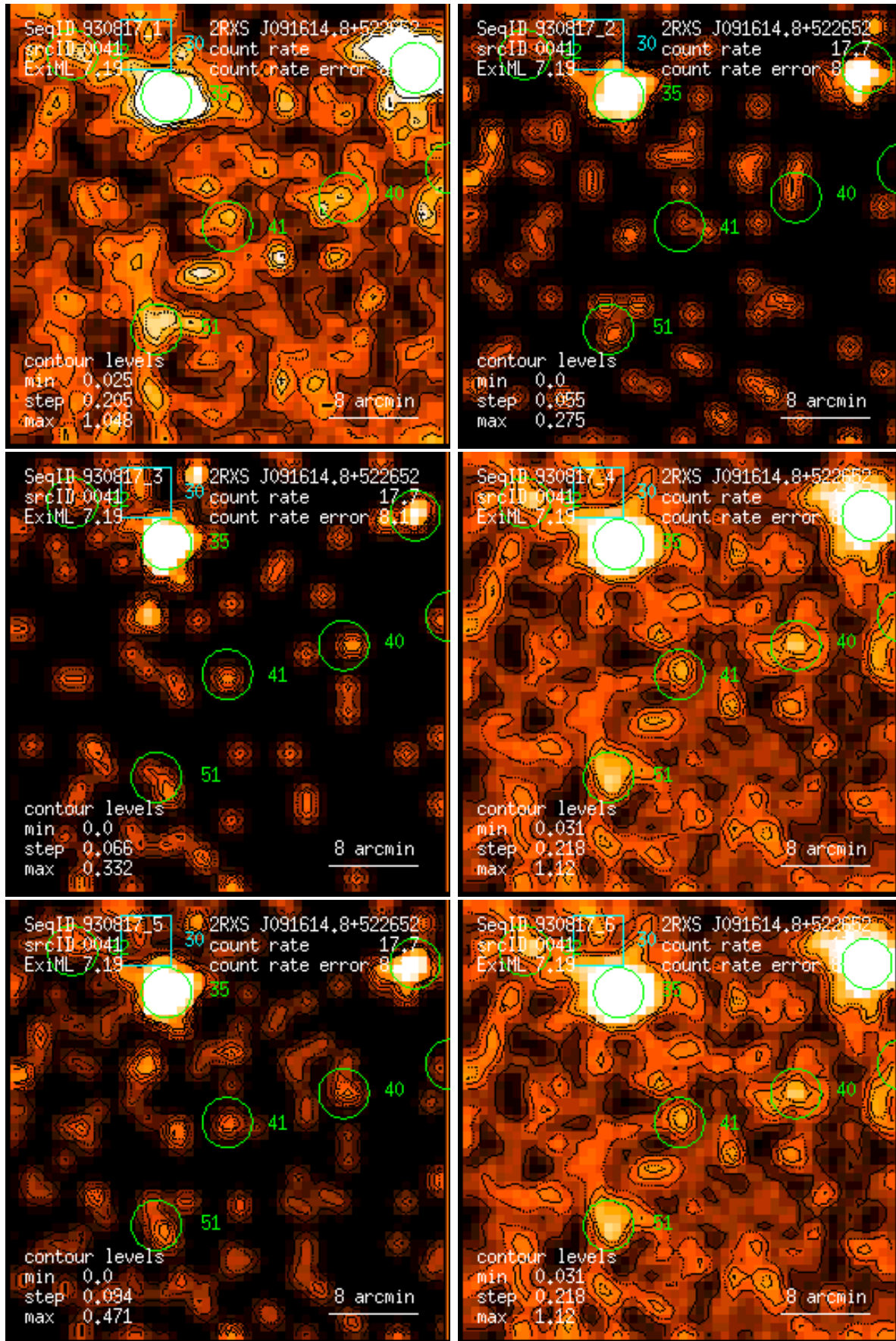
Figure 41: RASS 930817: detection 0041: band rate images, Gaussian filter: (1) PSPC channels 11 – 41, (2) 52 – 90, (3) 91 – 201, (4) 11 – 235, (5) 52 – 201, (6) 11 – 201. Broad band rates in counts/ks. Band rate contour levels in counts/ks/arcmin 2 .
