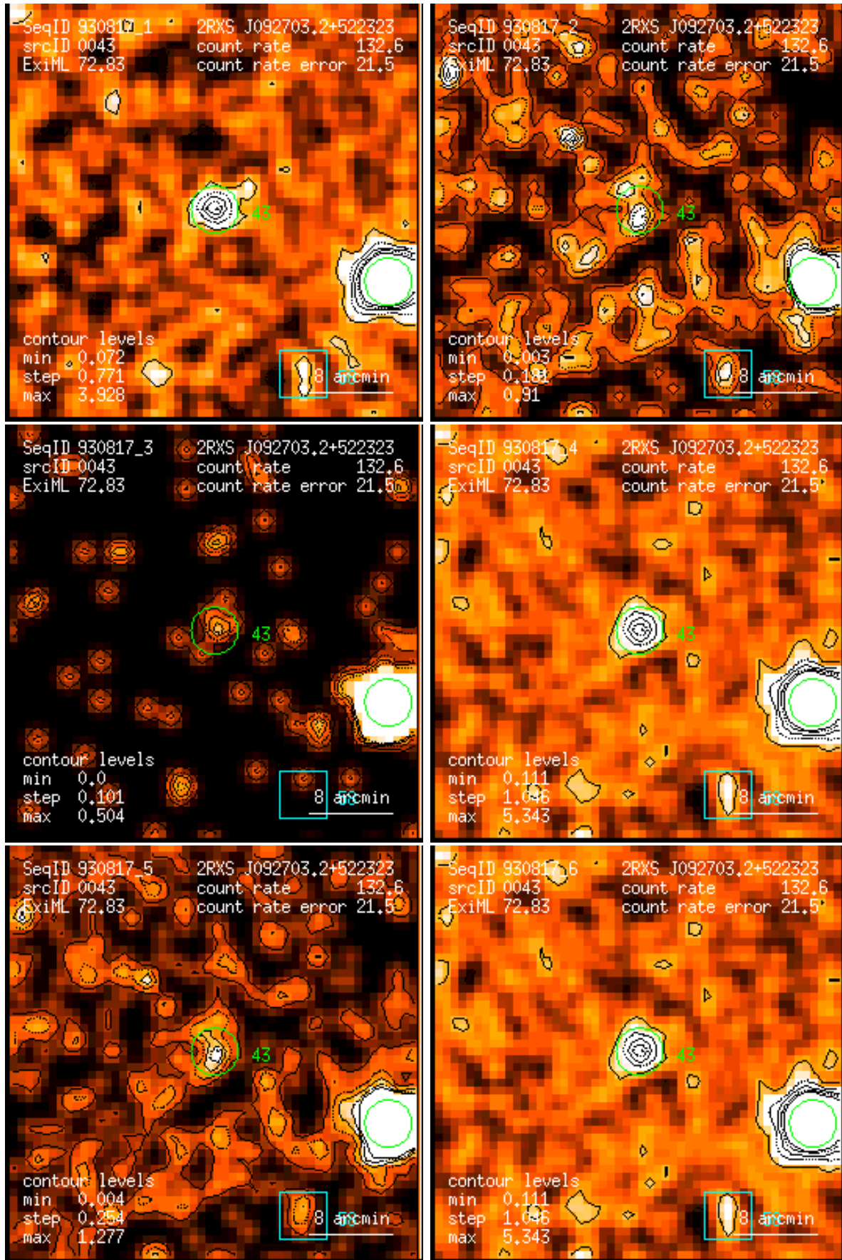
Figure 43: RASS 930817: detection 0043: band rate images, Gaussian filter: (1) PSPC channels 11 – 41, (2) 52 – 90, (3) 91 – 201, (4) 11 – 235, (5) 52 – 201, (6) 11 – 201. Broad band rates in counts/ks. Band rate contour levels in counts/ks/arcmin 2 .
