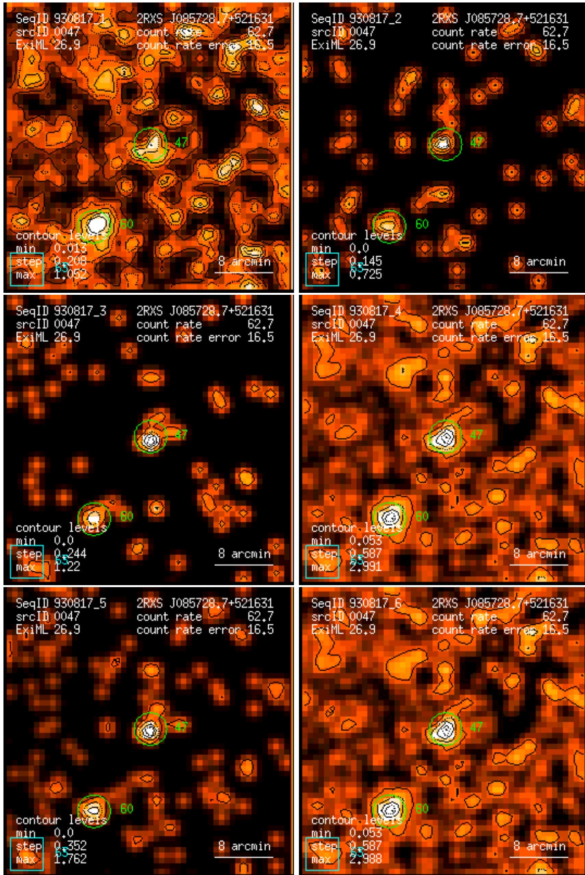
Figure 47: RASS 930817: detection 0047: band rate images, Gaussian filter: (1) PSPC channels 11 – 41, (2) 52 – 90, (3) 91 – 201, (4) 11 – 235, (5) 52 – 201, (6) 11 – 201. Broad band rates in counts/ks. Band rate contour levels in counts/ks/arcmin 2 .
