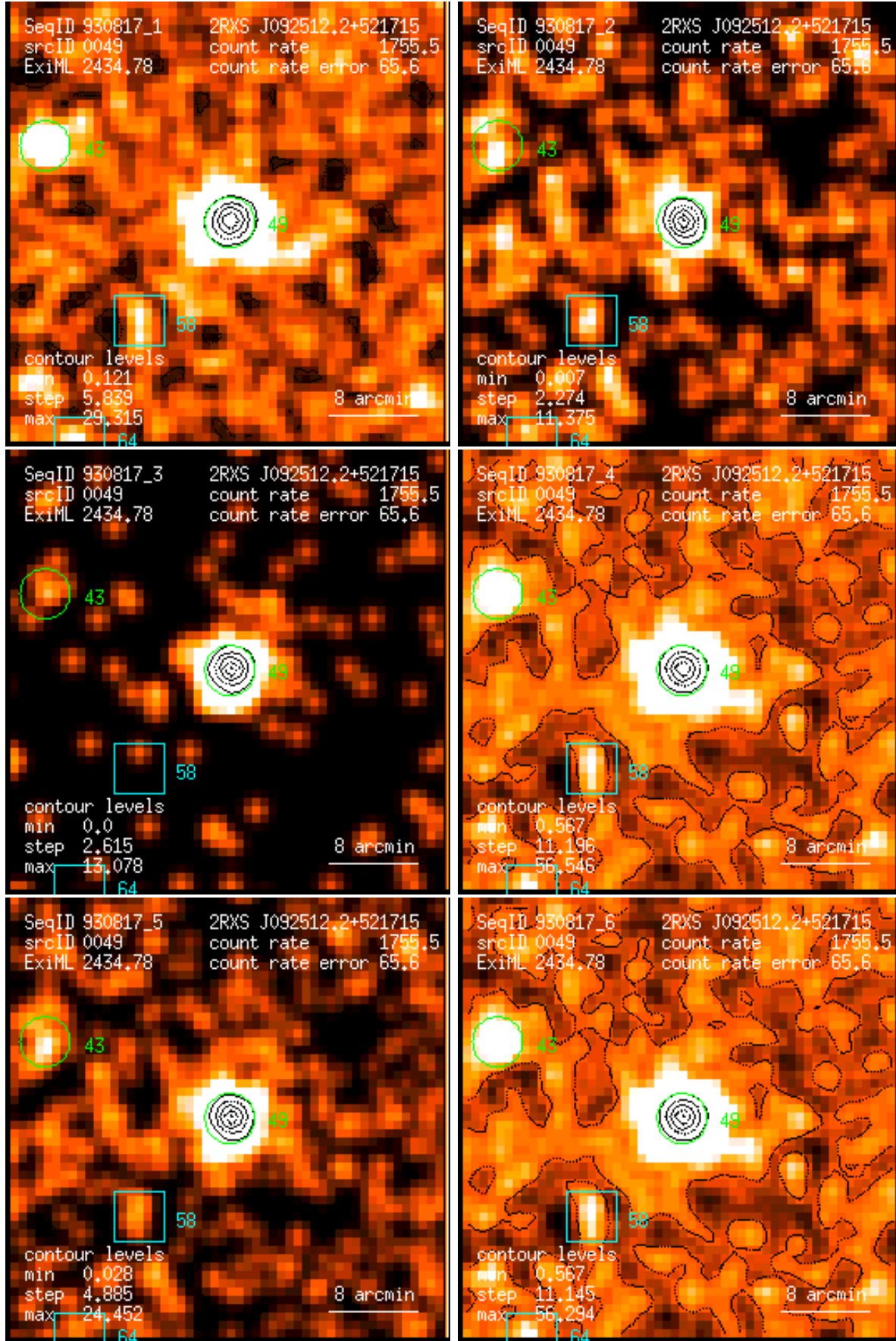
Figure 49: RASS 930817: detection 0049: band rate images, Gaussian filter: (1) PSPC channels 11 – 41, (2) 52 – 90, (3) 91 – 201, (4) 11 – 235, (5) 52 – 201, (6) 11 – 201. Broad band rates in counts/ks. Band rate contour levels in counts/ks/arcmin 2 .
