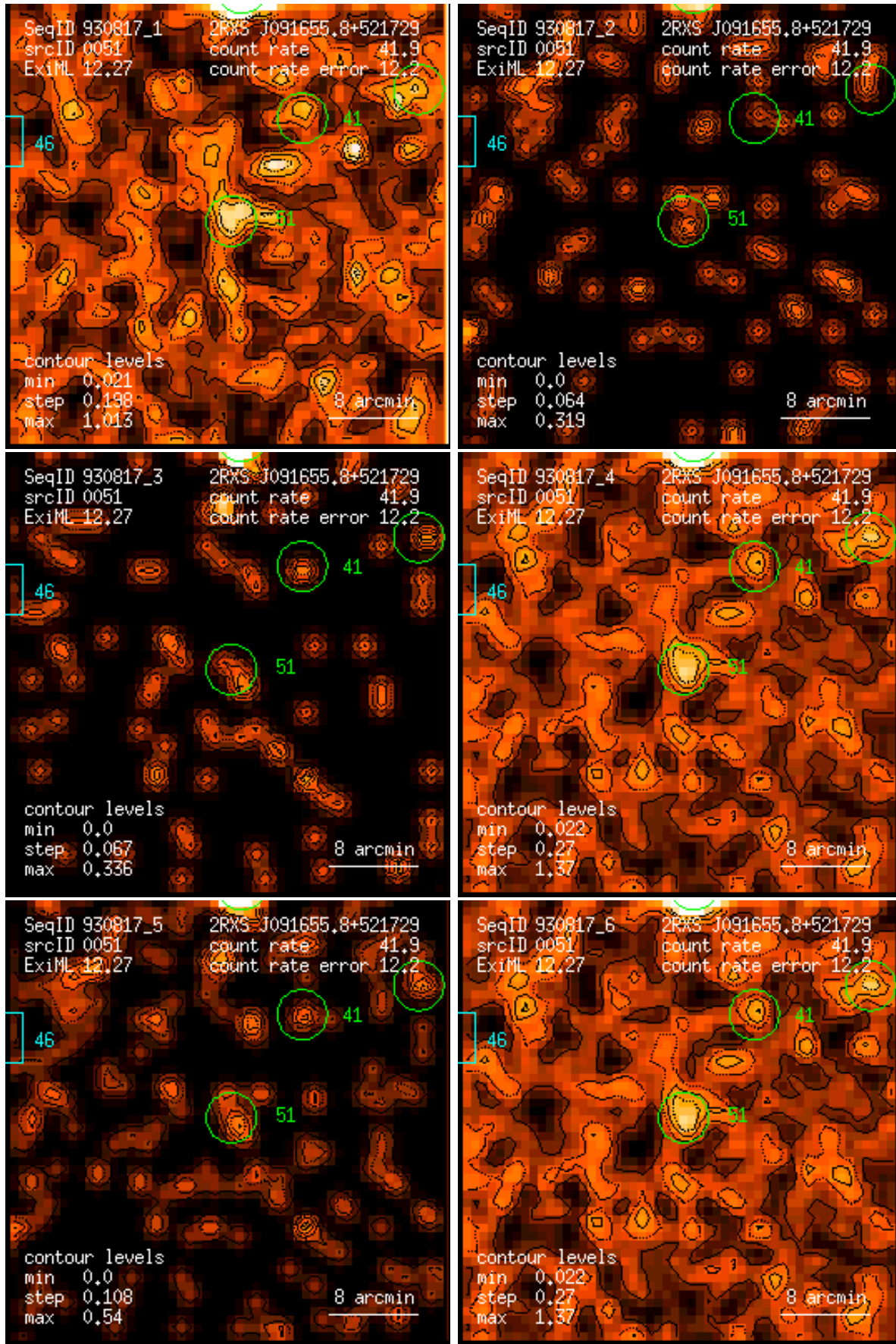
Figure 51: RASS 930817: detection 0051: band rate images, Gaussian filter: (1) PSPC channels 11 – 41, (2) 52 – 90, (3) 91 – 201, (4) 11 – 235, (5) 52 – 201, (6) 11 – 201. Broad band rates in counts/ks. Band rate contour levels in counts/ks/arcmin 2 .
