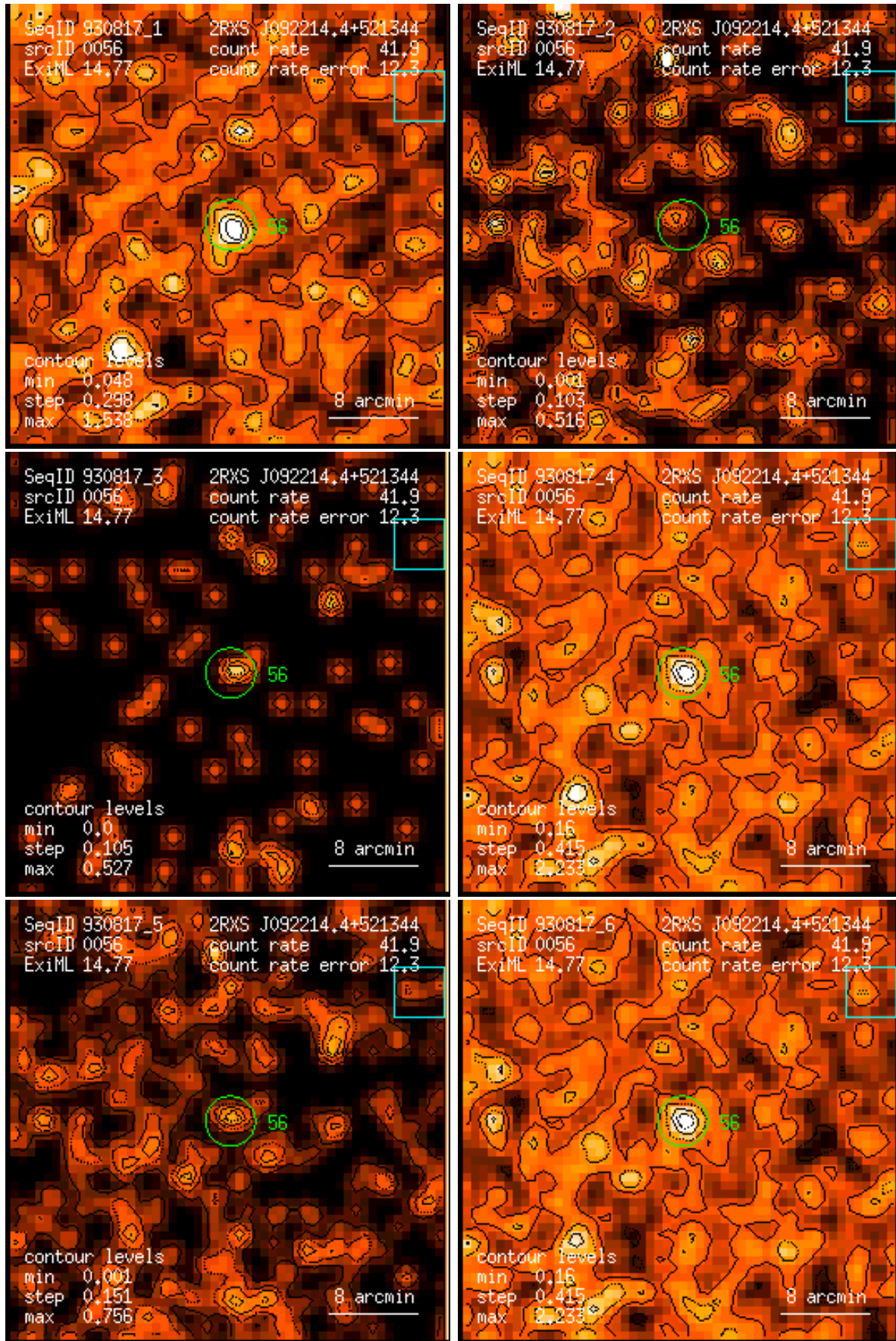
Figure 56: RASS 930817: detection 0056: band rate images, Gaussian filter: (1) PSPC channels 11 – 41, (2) 52 – 90, (3) 91 – 201, (4) 11 – 235, (5) 52 – 201, (6) 11 – 201. Broad band rates in counts/ks. Band rate contour levels in counts/ks/arcmin 2 .
