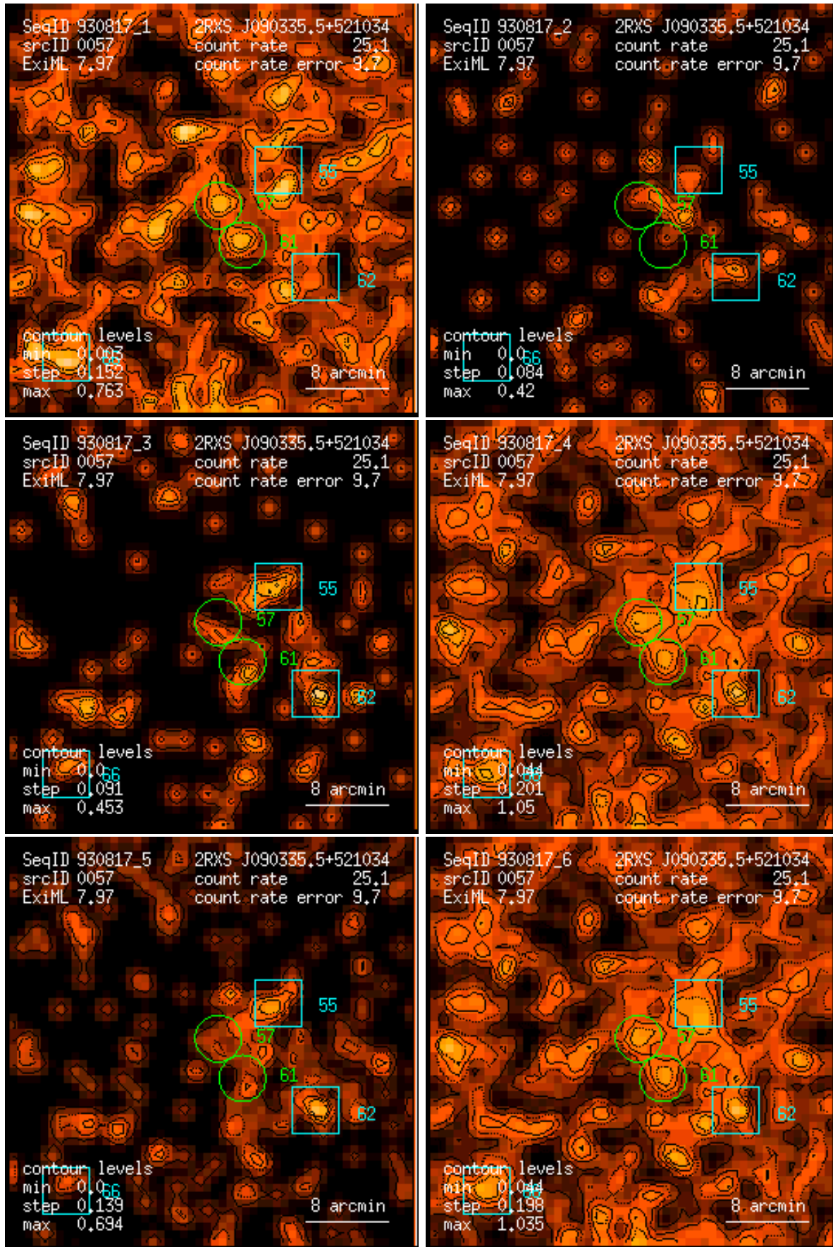
Figure 57: RASS 930817: detection 0057: band rate images, Gaussian filter: (1) PSPC channels 11 – 41, (2) 52 – 90, (3) 91 – 201, (4) 11 – 235, (5) 52 – 201, (6) 11 – 201. Broad band rates in counts/ks. Band rate contour levels in counts/ks/arcmin 2 .
