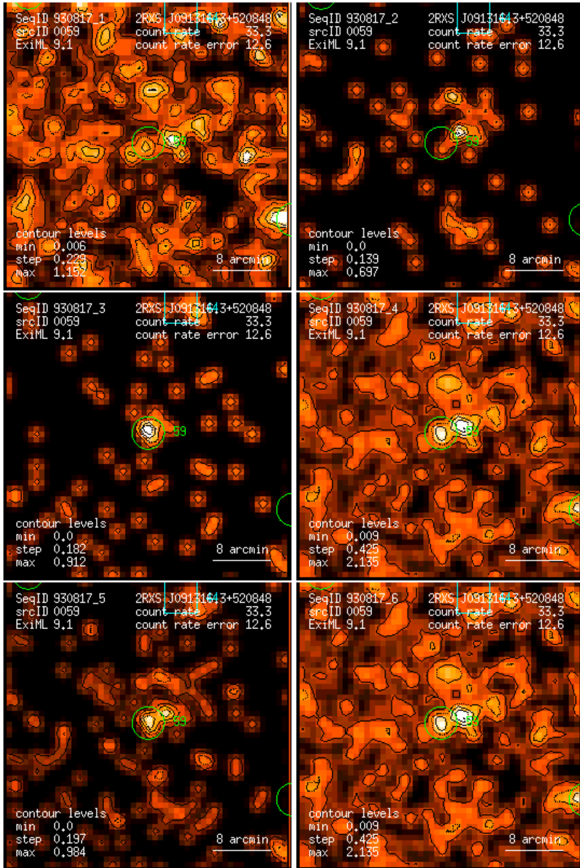
Figure 59: RASS 930817: detection 0059: band rate images, Gaussian filter: (1) PSPC channels 11 – 41, (2) 52 – 90, (3) 91 – 201, (4) 11 – 235, (5) 52 – 201, (6) 11 – 201. Broad band rates in counts/ks. Band rate contour levels in counts/ks/arcmin 2 .
