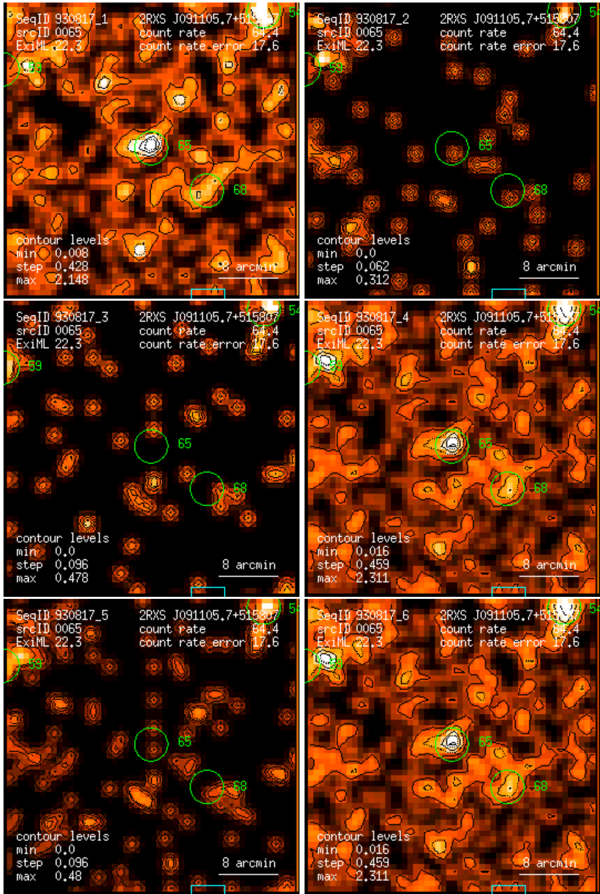
Figure 65: RASS 930817: detection 0065: band rate images, Gaussian filter: (1) PSPC channels 11 – 41, (2) 52 – 90, (3) 91 – 201, (4) 11 – 235, (5) 52 – 201, (6) 11 – 201. Broad band rates in counts/ks. Band rate contour levels in counts/ks/arcmin 2 .
