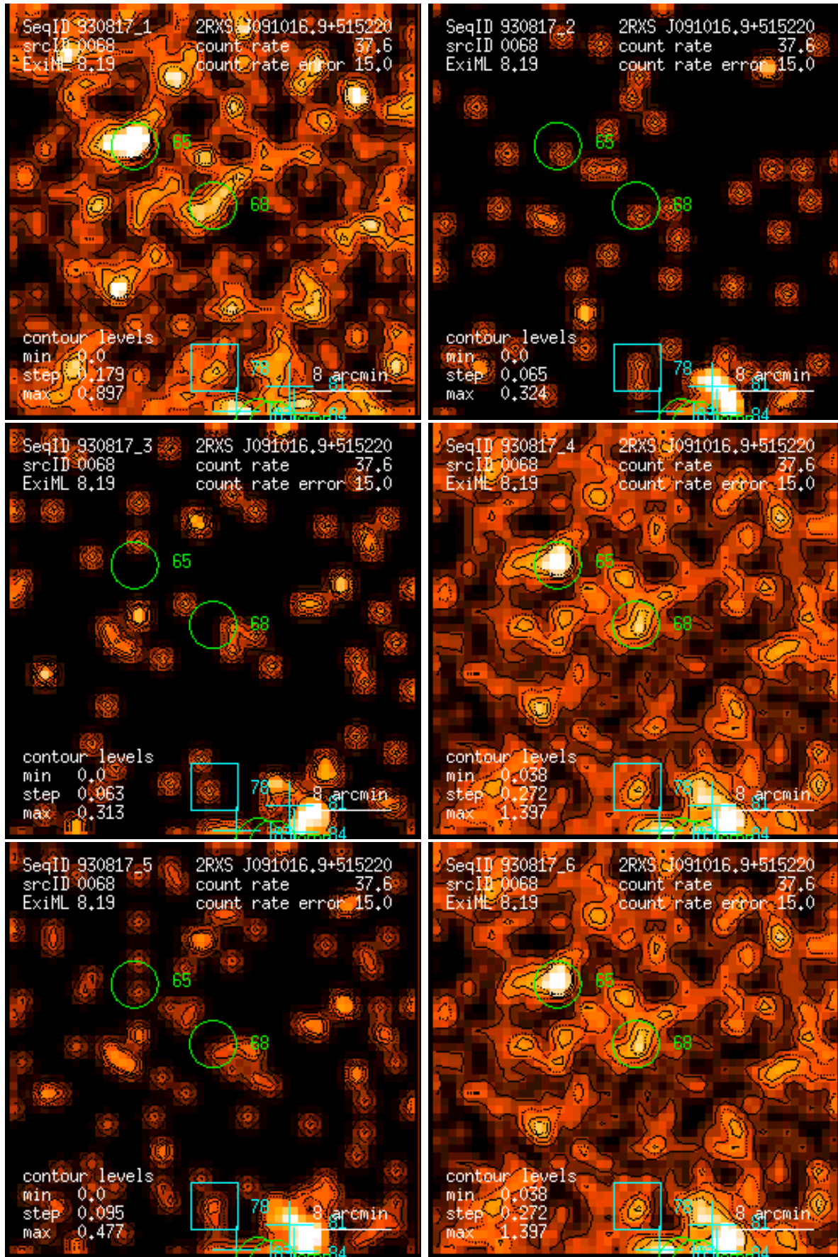
Figure 68: RASS 930817: detection 0068: band rate images, Gaussian filter: (1) PSPC channels 11 – 41, (2) 52 – 90, (3) 91 – 201, (4) 11 – 235, (5) 52 – 201, (6) 11 – 201. Broad band rates in counts/ks. Band rate contour levels in counts/ks/arcmin 2 .
