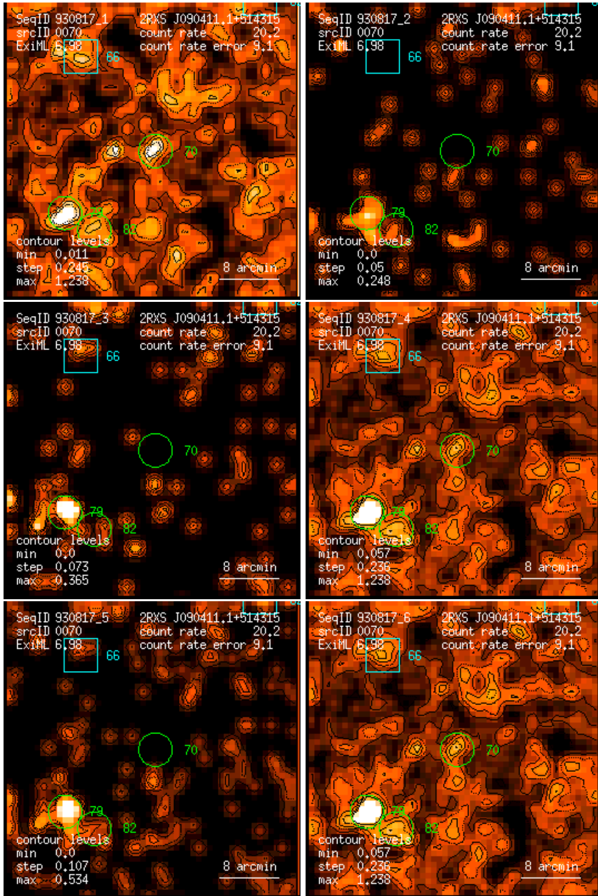
Figure 70: RASS 930817: detection 0070: band rate images, Gaussian filter: (1) PSPC channels 11 – 41, (2) 52 – 90, (3) 91 – 201, (4) 11 – 235, (5) 52 – 201, (6) 11 – 201. Broad band rates in counts/ks. Band rate contour levels in counts/ks/arcmin 2 .
