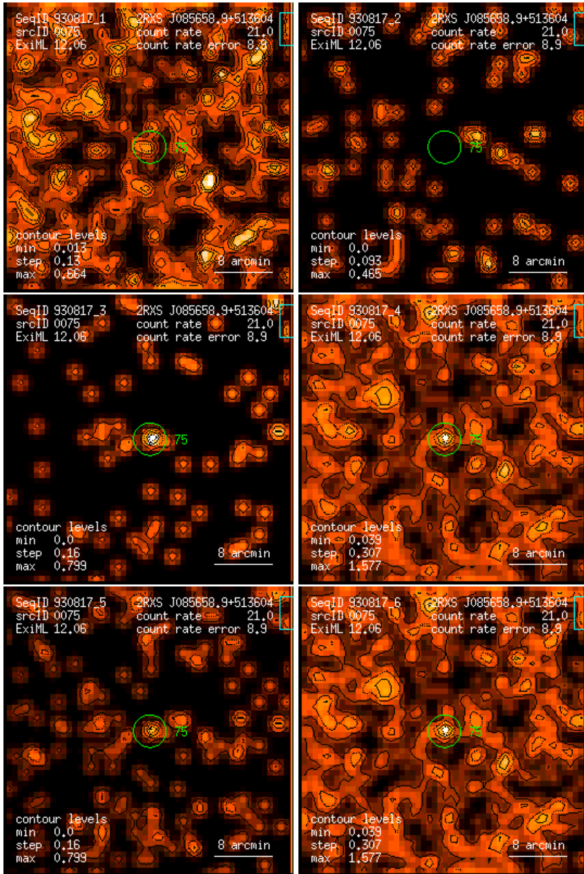
Figure 75: RASS 930817: detection 0075: band rate images, Gaussian filter: (1) PSPC channels 11 – 41, (2) 52 – 90, (3) 91 – 201, (4) 11 – 235, (5) 52 – 201, (6) 11 – 201. Broad band rates in counts/ks. Band rate contour levels in counts/ks/arcmin 2 .
