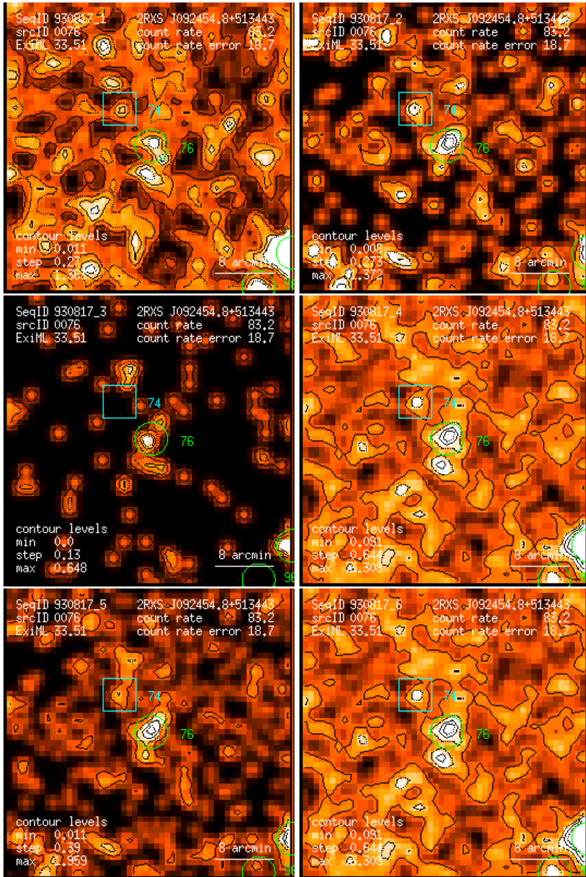
Figure 76: RASS 930817: detection 0076: band rate images, Gaussian filter: (1) PSPC channels 11 – 41, (2) 52 – 90, (3) 91 – 201, (4) 11 – 235, (5) 52 – 201, (6) 11 – 201. Broad band rates in counts/ks. Band rate contour levels in counts/ks/arcmin 2 .
