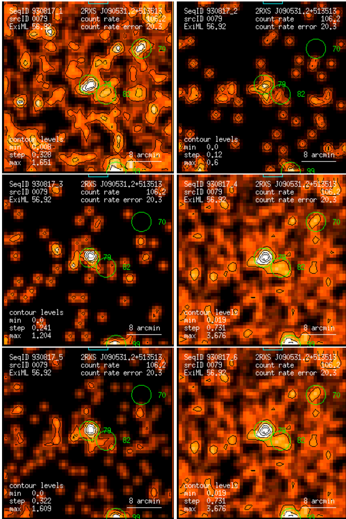
Figure 79: RASS 930817: detection 0079: band rate images, Gaussian filter: (1) PSPC channels 11 – 41, (2) 52 – 90, (3) 91 – 201, (4) 11 – 235, (5) 52 – 201, (6) 11 – 201. Broad band rates in counts/ks. Band rate contour levels in counts/ks/arcmin 2 .
