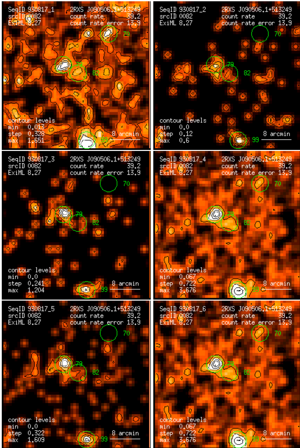
Figure 82: RASS 930817: detection 0082: band rate images, Gaussian filter: (1) PSPC channels 11 – 41, (2) 52 – 90, (3) 91 – 201, (4) 11 – 235, (5) 52 – 201, (6) 11 – 201. Broad band rates in counts/ks. Band rate contour levels in counts/ks/arcmin 2 .
