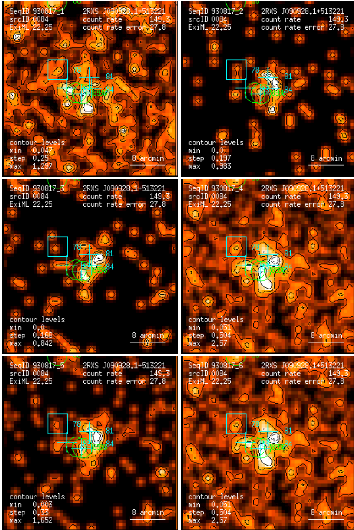
Figure 84: RASS 930817: detection 0084: band rate images, Gaussian filter: (1) PSPC channels 11 – 41, (2) 52 – 90, (3) 91 – 201, (4) 11 – 235, (5) 52 – 201, (6) 11 – 201. Broad band rates in counts/ks. Band rate contour levels in counts/ks/arcmin 2 .
