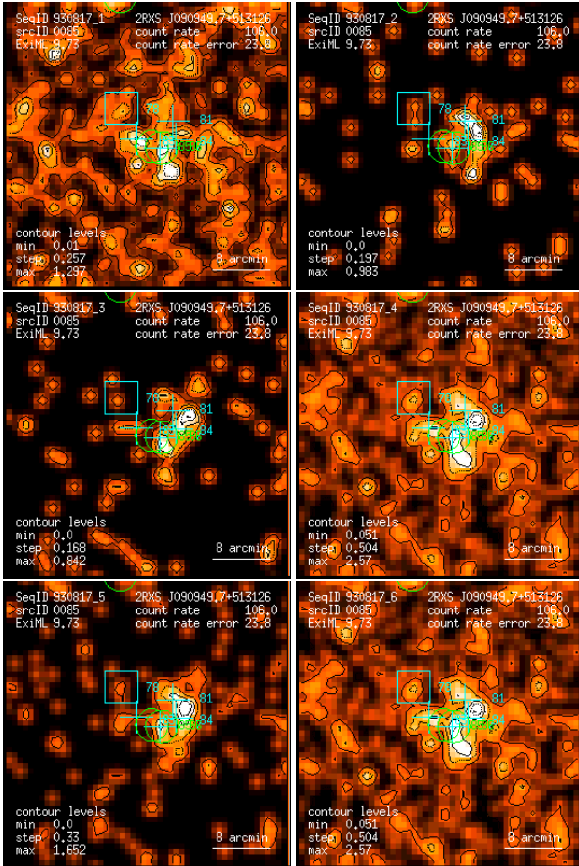
Figure 85: RASS 930817: detection 0085: band rate images, Gaussian filter: (1) PSPC channels 11 – 41, (2) 52 – 90, (3) 91 – 201, (4) 11 – 235, (5) 52 – 201, (6) 11 – 201. Broad band rates in counts/ks. Band rate contour levels in counts/ks/arcmin 2 .
