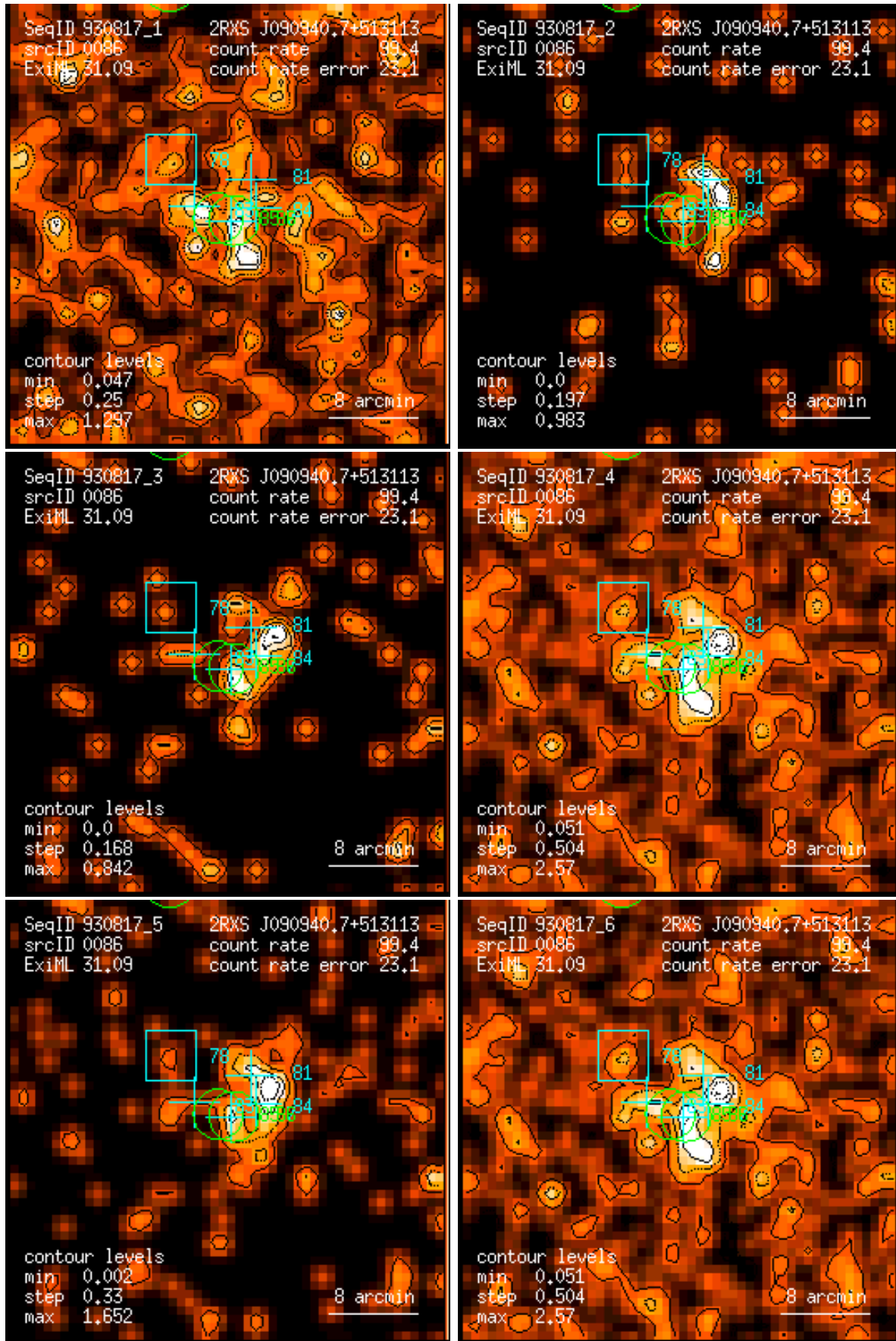
Figure 86: RASS 930817: detection 0086: band rate images, Gaussian filter: (1) PSPC channels 11 – 41, (2) 52 – 90, (3) 91 – 201, (4) 11 – 235, (5) 52 – 201, (6) 11 – 201. Broad band rates in counts/ks. Band rate contour levels in counts/ks/arcmin 2 .
