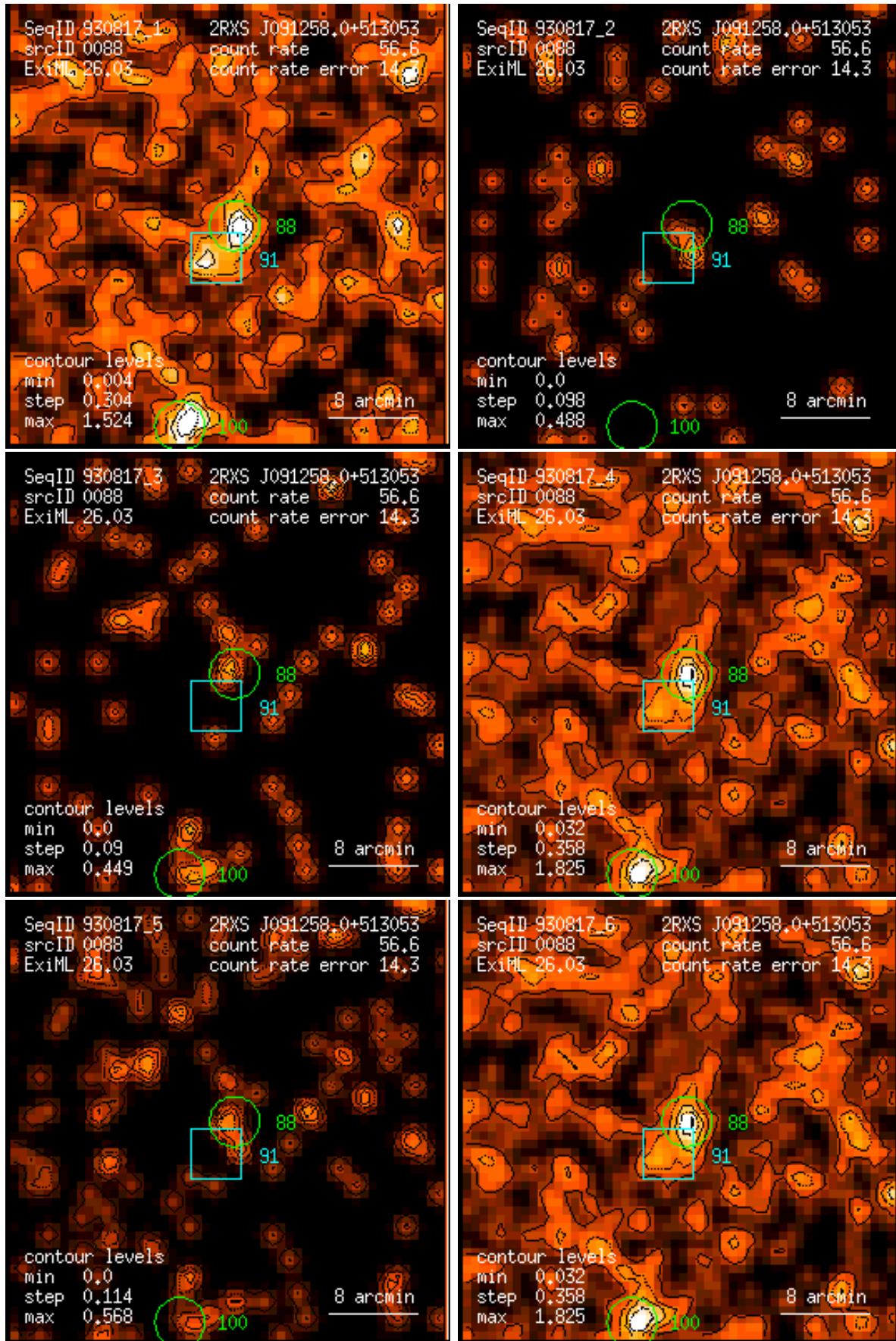
Figure 88: RASS 930817: detection 0088: band rate images, Gaussian filter: (1) PSPC channels 11 – 41, (2) 52 – 90, (3) 91 – 201, (4) 11 – 235, (5) 52 – 201, (6) 11 – 201. Broad band rates in counts/ks. Band rate contour levels in counts/ks/arcmin 2 .
