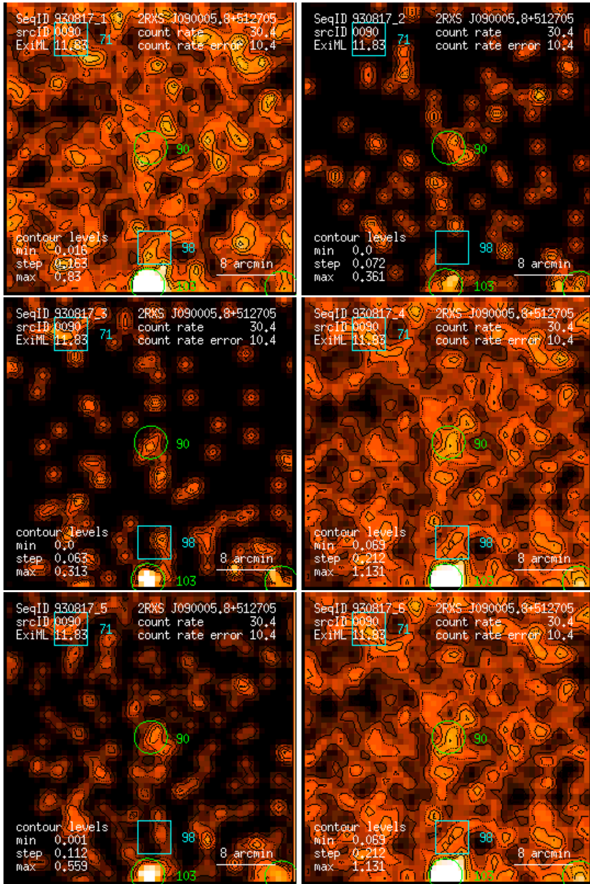
Figure 90: RASS 930817: detection 0090: band rate images, Gaussian filter: (1) PSPC channels 11 – 41, (2) 52 – 90, (3) 91 – 201, (4) 11 – 235, (5) 52 – 201, (6) 11 – 201. Broad band rates in counts/ks. Band rate contour levels in counts/ks/arcmin 2 .
