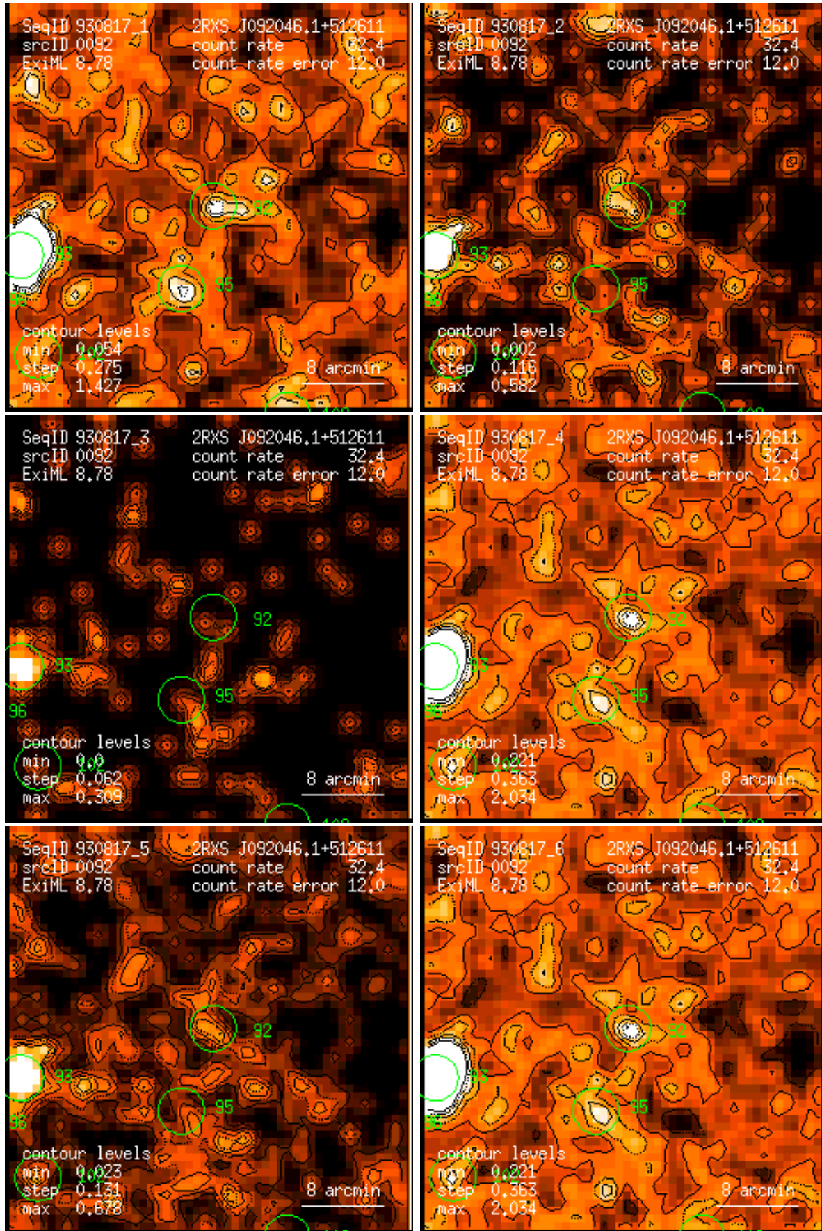
Figure 92: RASS 930817: detection 0092: band rate images, Gaussian filter: (1) PSPC channels 11 – 41, (2) 52 – 90, (3) 91 – 201, (4) 11 – 235, (5) 52 – 201, (6) 11 – 201. Broad band rates in counts/ks. Band rate contour levels in counts/ks/arcmin 2 .
