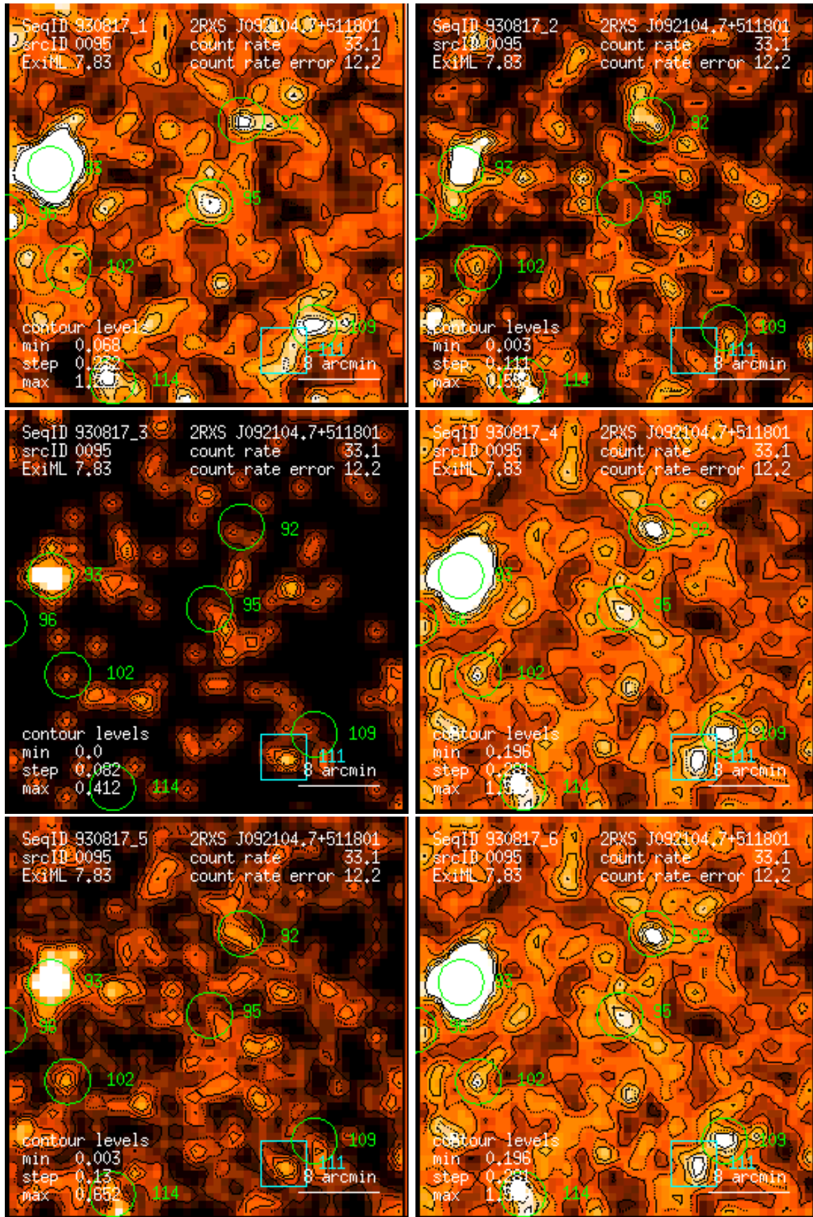
Figure 95: RASS 930817: detection 0095: band rate images, Gaussian filter: (1) PSPC channels 11 – 41, (2) 52 – 90, (3) 91 – 201, (4) 11 – 235, (5) 52 – 201, (6) 11 – 201. Broad band rates in counts/ks. Band rate contour levels in counts/ks/arcmin 2 .
