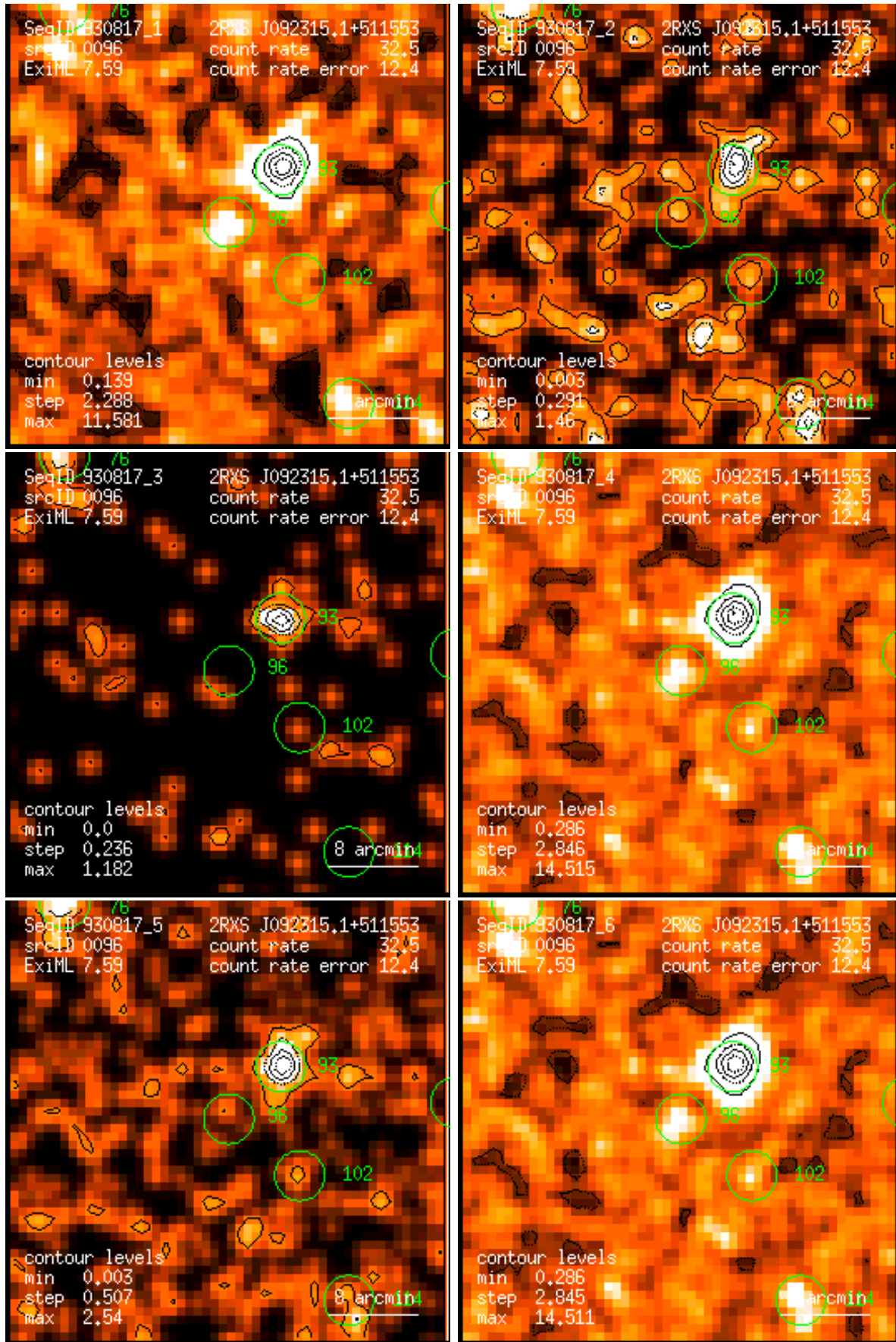
Figure 96: RASS 930817: detection 0096: band rate images, Gaussian filter: (1) PSPC channels 11 – 41, (2) 52 – 90, (3) 91 – 201, (4) 11 – 235, (5) 52 – 201, (6) 11 – 201. Broad band rates in counts/ks. Band rate contour levels in counts/ks/arcmin 2 .
