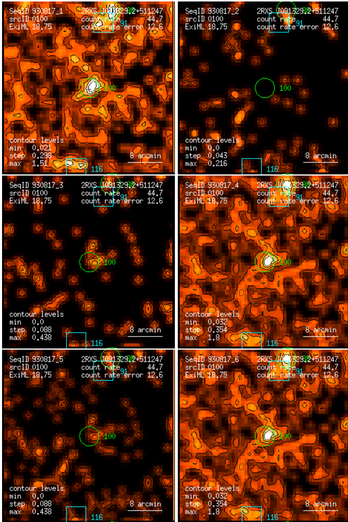
Figure 100: RASS 930817: detection 0100: band rate images, Gaussian filter: (1) PSPC channels 11 – 41, (2) 52 – 90, (3) 91 – 201, (4) 11 – 235, (5) 52 – 201, (6) 11 – 201. Broad band rates in counts/ks. Band rate contour levels in counts/ks/arcmin 2 .
