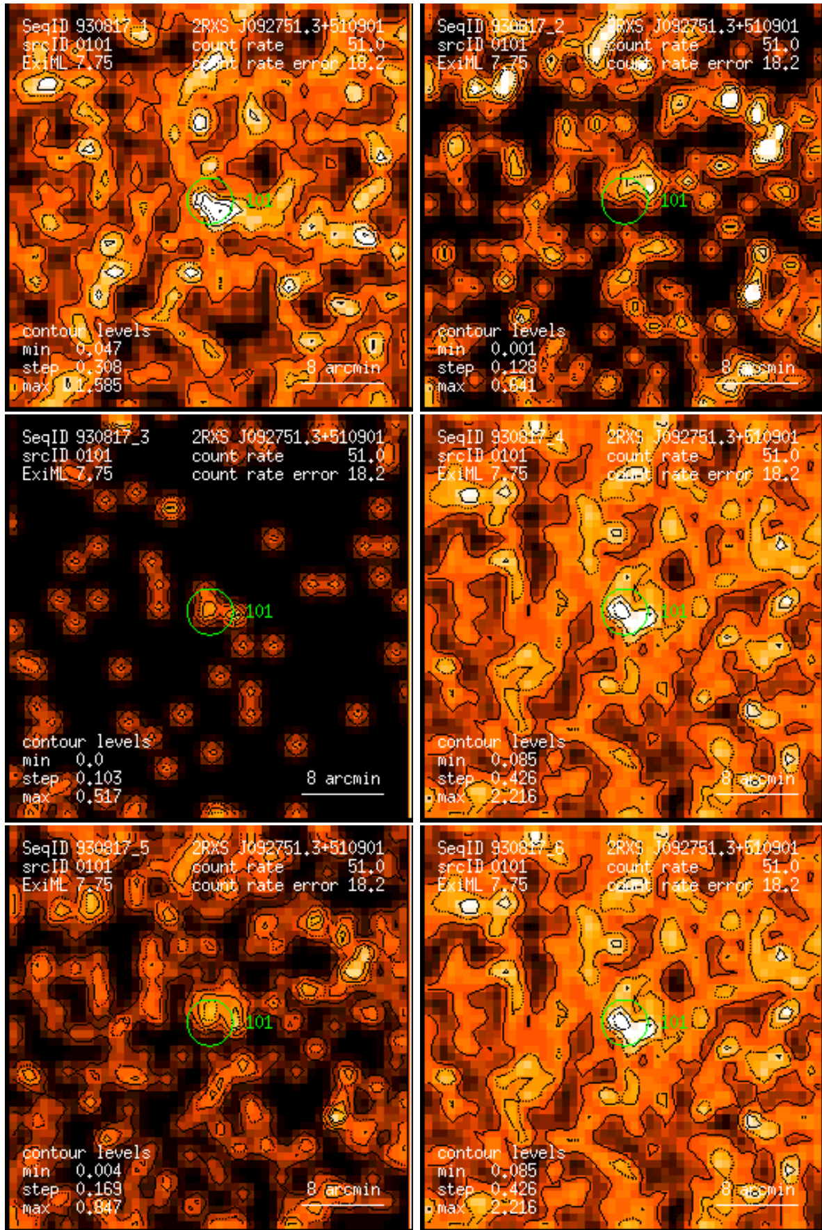
Figure 101: RASS 930817: detection 0101: band rate images, Gaussian filter: (1) PSPC channels 11 – 41, (2) 52 – 90, (3) 91 – 201, (4) 11 – 235, (5) 52 – 201, (6) 11 – 201. Broad band rates in counts/ks. Band rate contour levels in counts/ks/arcmin 2 .
