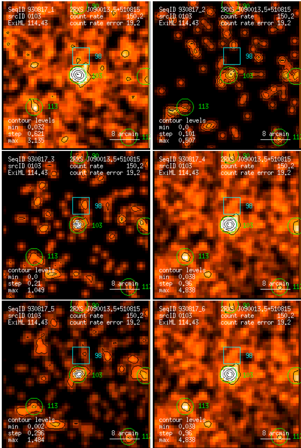
Figure 103: RASS 930817: detection 0103: band rate images, Gaussian filter: (1) PSPC channels 11 – 41, (2) 52 – 90, (3) 91 – 201, (4) 11 – 235, (5) 52 – 201, (6) 11 – 201. Broad band rates in counts/ks. Band rate contour levels in counts/ks/arcmin 2 .
