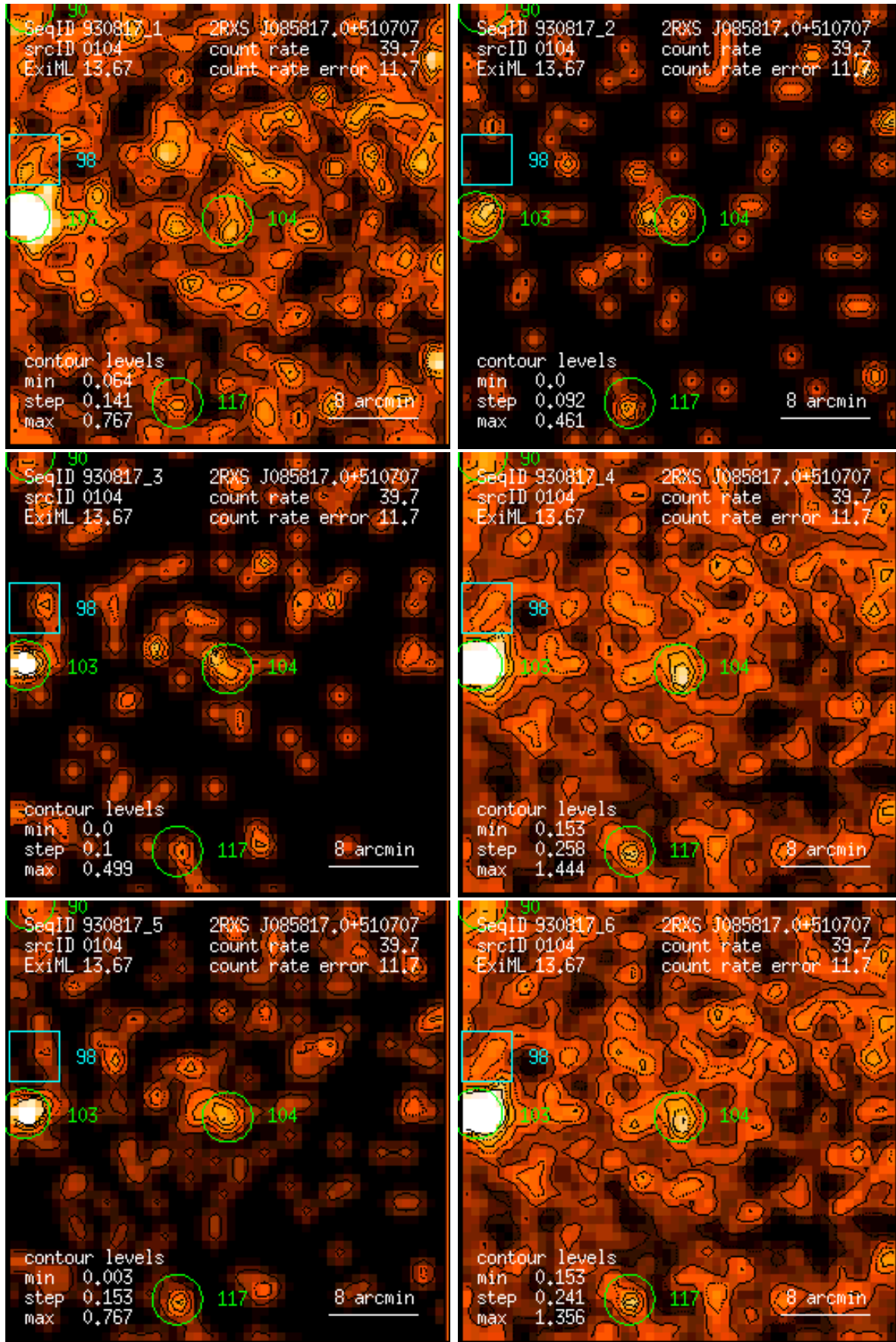
Figure 104: RASS 930817: detection 0104: band rate images, Gaussian filter: (1) PSPC channels 11 – 41, (2) 52 – 90, (3) 91 – 201, (4) 11 – 235, (5) 52 – 201, (6) 11 – 201. Broad band rates in counts/ks. Band rate contour levels in counts/ks/arcmin 2 .
