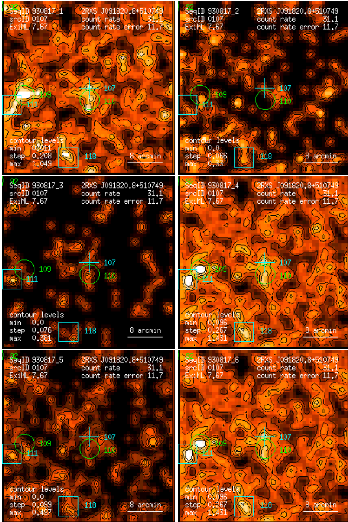
Figure 107: RASS 930817: detection 0107: band rate images, Gaussian filter: (1) PSPC channels 11 – 41, (2) 52 – 90, (3) 91 – 201, (4) 11 – 235, (5) 52 – 201, (6) 11 – 201. Broad band rates in counts/ks. Band rate contour levels in counts/ks/arcmin 2 .
