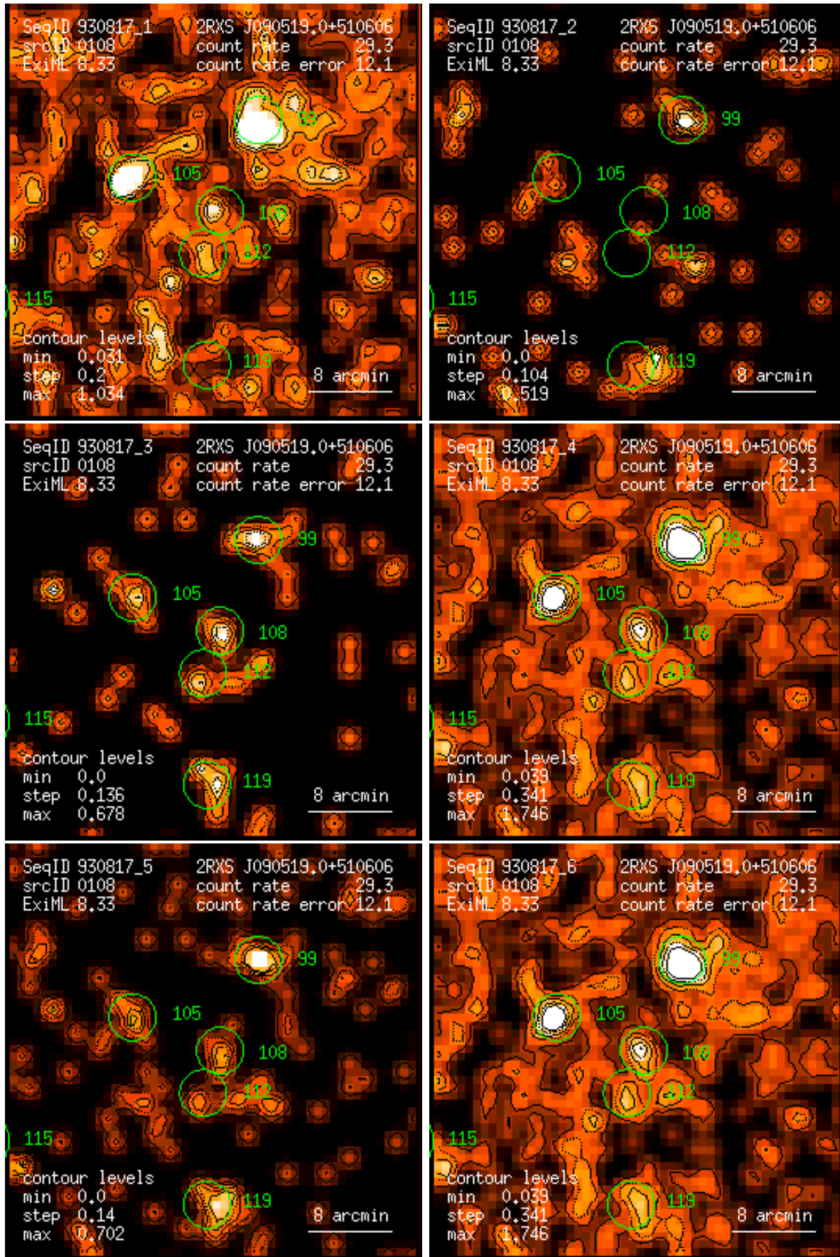
Figure 108: RASS 930817: detection 0108: band rate images, Gaussian filter: (1) PSPC channels 11 – 41, (2) 52 – 90, (3) 91 – 201, (4) 11 – 235, (5) 52 – 201, (6) 11 – 201. Broad band rates in counts/ks. Band rate contour levels in counts/ks/arcmin 2 .
