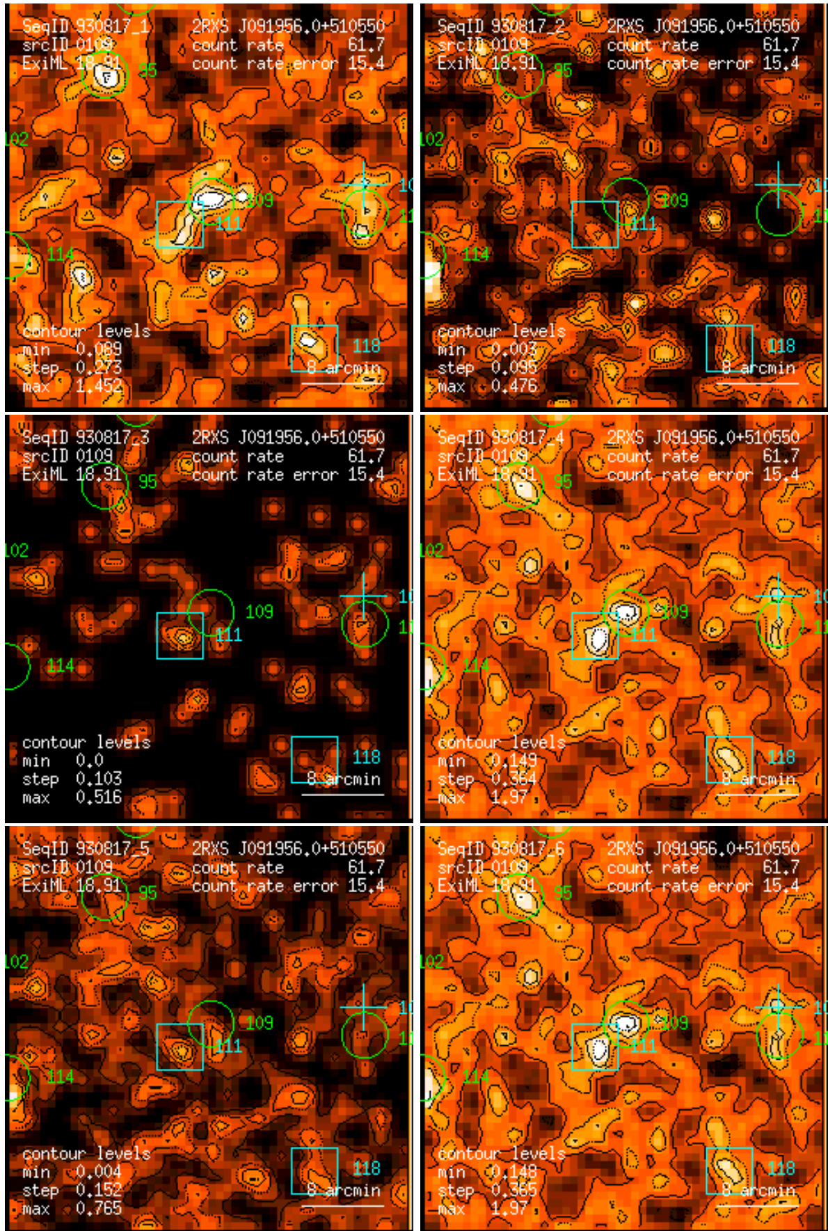
Figure 109: RASS 930817: detection 0109: band rate images, Gaussian filter: (1) PSPC channels 11 – 41, (2) 52 – 90, (3) 91 – 201, (4) 11 – 235, (5) 52 – 201, (6) 11 – 201. Broad band rates in counts/ks. Band rate contour levels in counts/ks/arcmin 2 .
