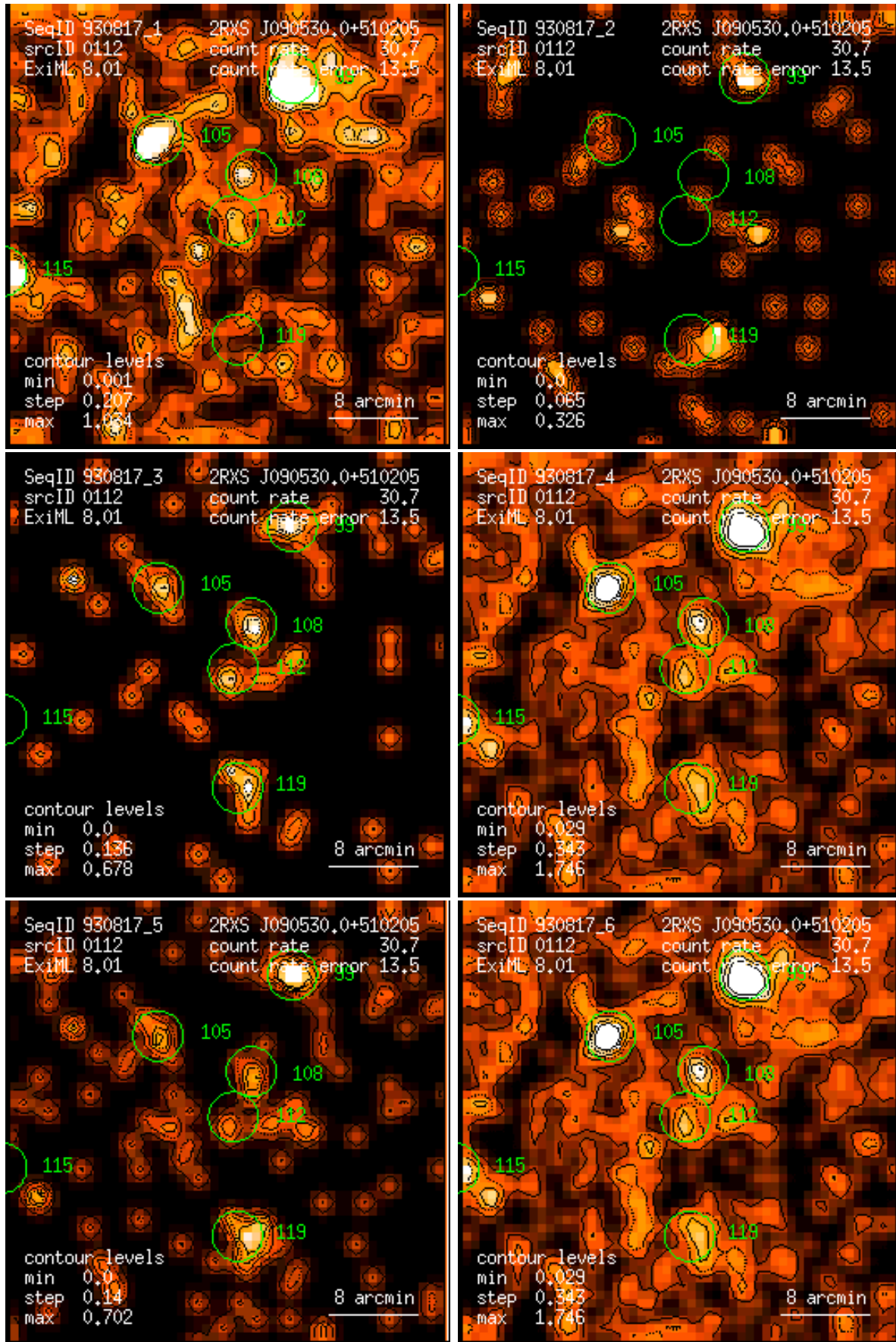
Figure 112: RASS 930817: detection 0112: band rate images, Gaussian filter: (1) PSPC channels 11 – 41, (2) 52 – 90, (3) 91 – 201, (4) 11 – 235, (5) 52 – 201, (6) 11 – 201. Broad band rates in counts/ks. Band rate contour levels in counts/ks/arcmin 2 .
