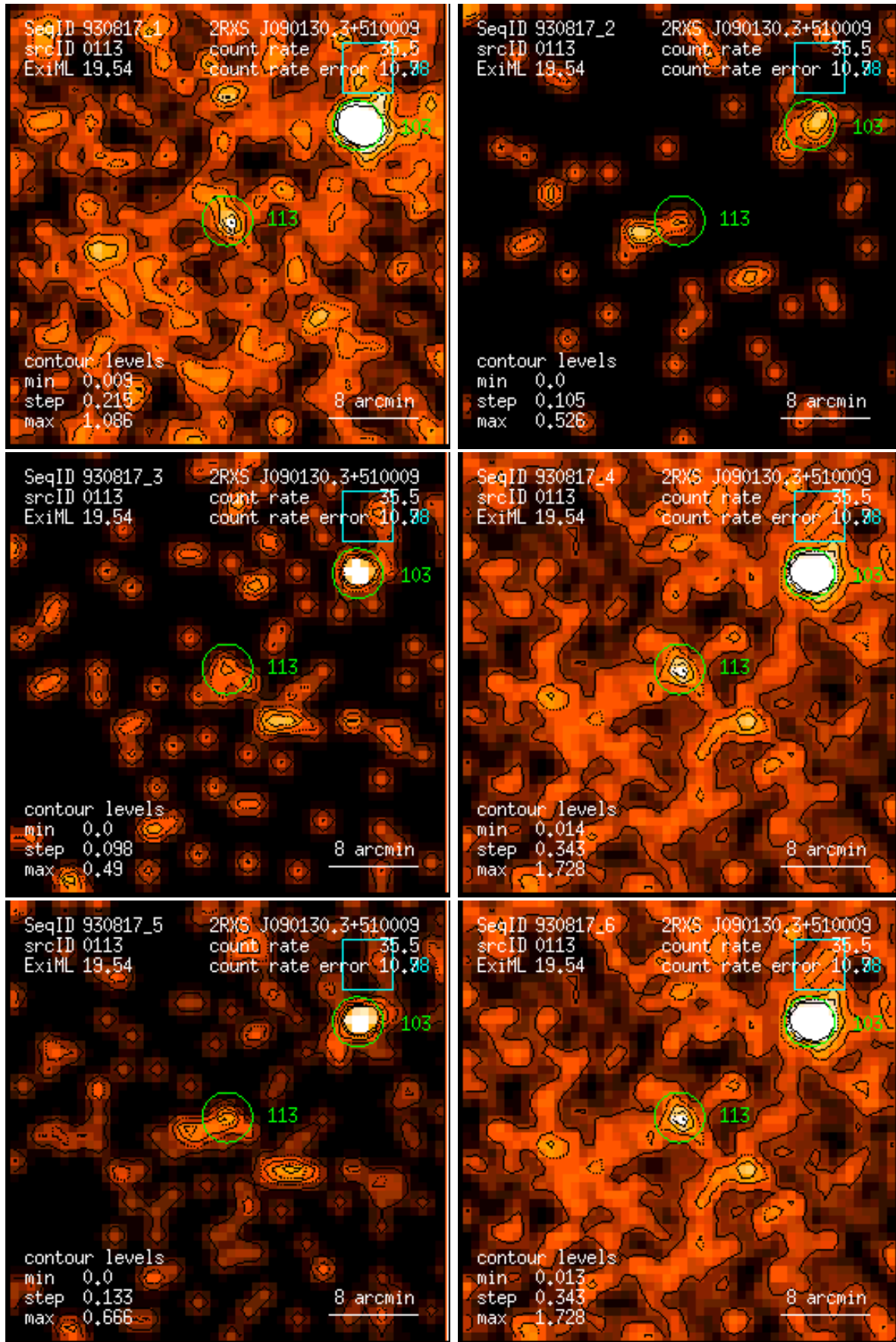
Figure 113: RASS 930817: detection 0113: band rate images, Gaussian filter: (1) PSPC channels 11 – 41, (2) 52 – 90, (3) 91 – 201, (4) 11 – 235, (5) 52 – 201, (6) 11 – 201. Broad band rates in counts/ks. Band rate contour levels in counts/ks/arcmin 2 .
